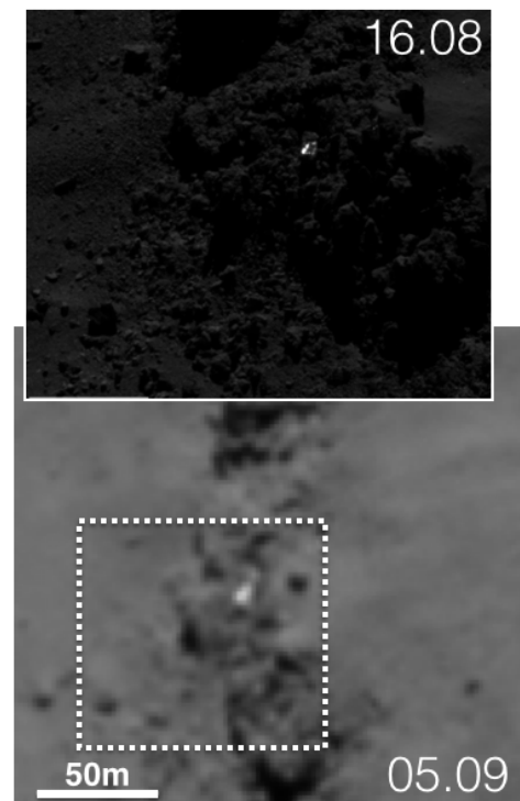
Fig. 5. Effect of the spatial resolution on the aspect of surface bright features. In both examples shown here, the surface shown at higher resolution allows resolving small meter-sized bright spots inside what looks like homogeneous bright regions at lower scale. As a result, the bright spots are much smaller and brighter than what could be inferred from the earlier lower resolution observation. a) Imhotep. Subset of OSIRIS NAC images: NAC_2014-08-16T19.59.14.556Z_ID30_1397549300_F22.IMG NAC_2014-09-30T20.44.47.569Z_ID30_1397549300_F22.IMG; b) Hatmehit. Subset of OSIRIS NAC images: NAC_2014-08-16T15.59.14.568Z_ID30_1397549500_F22.IMG NAC_2014-09-05T08.00.55.651Z_ID30_1397549500_F22.IMG.
