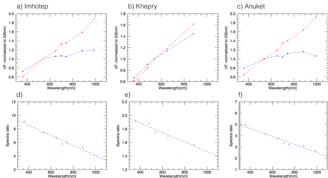
Fig. 9. a) , b) , and c) average normalized reflectance spectra of three different bright features (blue) and dark terrain nearby (red) for the examples shown in Figs. 7e, c, and a, respectively. Spectra of the bright features were averaged over a region of interest (ROI) of a few pixels defined inside the bright feature, avoiding its edges that are often affected by imperfect coregistration at the pixel scale. Spectra of the dark soil were averaged in a similar way over regions defined by avoiding all visible shadows in the image. All spectra were then normalized by their value of reflectance at 535.7 nm. d) , e) , and f) corresponding ratios between the average spectra of the bright feature and the average spectra of the dark soil (crosses) and linear fit through these points (dashed lines).
