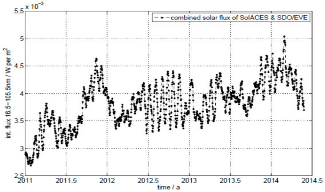
Figure 7: Combined EUV data set from the SDO/EVE and SOLAR/SolACES instruments covering the spectral range of 16.5-105.5 nm and a period of 3.5 years.
