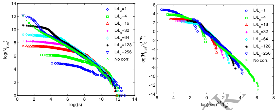
Fig. 8. IP accounting for the effect of in-plane curvature, \delta = 0.25 . Left: cumulative cluster size distribution; Right: collapse of the curves.
