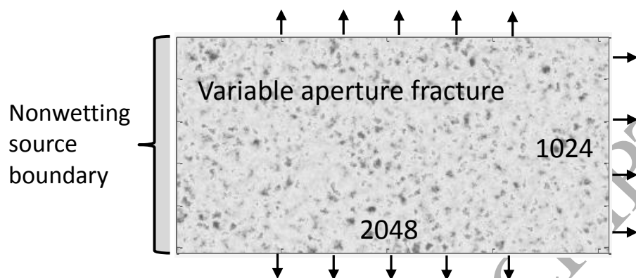
Fig. 2. Schematic of the modeling scenario. The variable aperture fracture is initially fully saturated with the wetting phase. The nonwetting fluid is invading from the left edge, and the wetting fluid is displaced and allowed to leave the fracture through the top, bottom and right edge.
