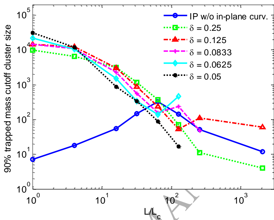
Fig. 10. Cutoff cluster size at 90% of total trapped mass (from large cluster end).
