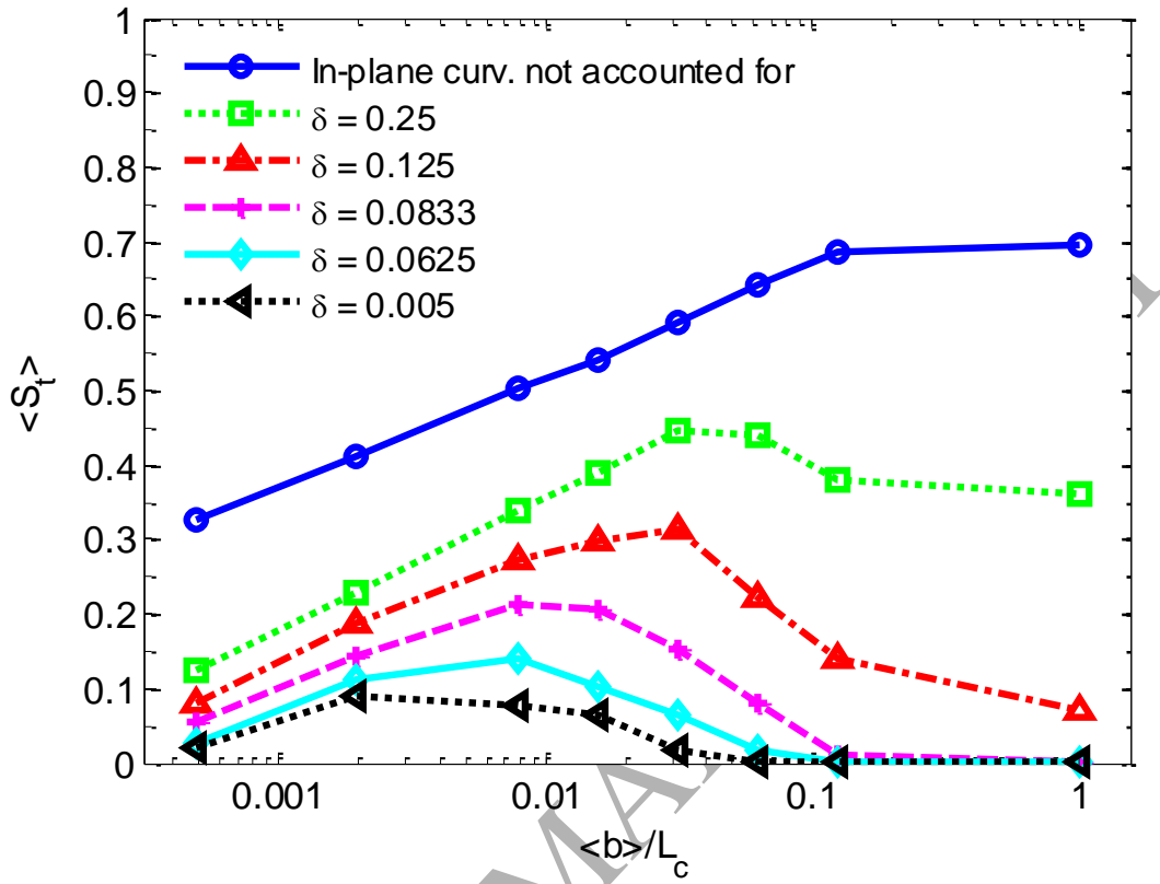
Fig. 5. Average trapped phase saturation \langle S_t \rangle as a function of the aperture correlation scale L_c and for different coefficients of variation \delta . The IP limit corresponds to the a simulation for which the in-plane curvature has not been accounted for when computing capillary pressures.
