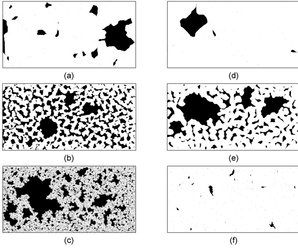
Fig. 4. Spatial distribution of the trapped wetting fluid (shown in black) for the aperture fields shown in Fig. 3 . The domain length L is 20.48 cm. (a) Coefficient of variation \delta = 0.25 , mismatch wave number L/L_c = 1 ; (b) \delta = 0.25 , L/L_c = 16 ; (c) \delta = 0.25 , L/L_c = 256 ; (d) \delta = 0.0833 , L/L_c = 1 ; (e) \delta = 0.0833 , L/L_c = 16 ; (f) \delta = 0.0833 , L/L_c = 256 .
