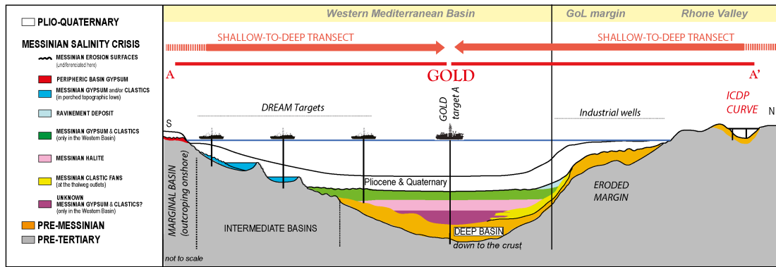
Figure 2 - Composite line drawing cross-section showing the markers of the MSC (modified from Lofi, et al., 2011;
