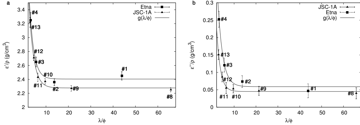
Fig. 5. Real part a) and imaginary part b) of the permittivity \epsilon normalized by the bulk density ( \text{g/cm}^3 ) as a function of the ratio of the wavelength (corresponding to the frequency of 190 GHz) to the mean grain \phi size for Etna and JSC-1A subsamples. The solid lines represent the exponential regressions of the measured points, expressed as g(\lambda/\phi) = a \times e^{(\lambda/\phi) \times b} + c . Panel a) : a equal to 4.13 \pm 1.72 and 3.75 \pm 0.61 ; b equal to -0.51 \pm 0.13 and -0.48 \pm 0.05 ; c equal to 2.40 \pm 0.05 and 2.28 \pm 0.02 , for the Etna and the JSC-1A subsamples, respectively. Panel b) : a equal to 0.80 \pm 0.34 and 0.59 \pm 0.14 ; b equal to -0.45 \pm 0.13 and -0.59 \pm 0.08 ; c equal to 0.06 \pm 0.01 and 0.050 \pm 0.003 , respectively.
