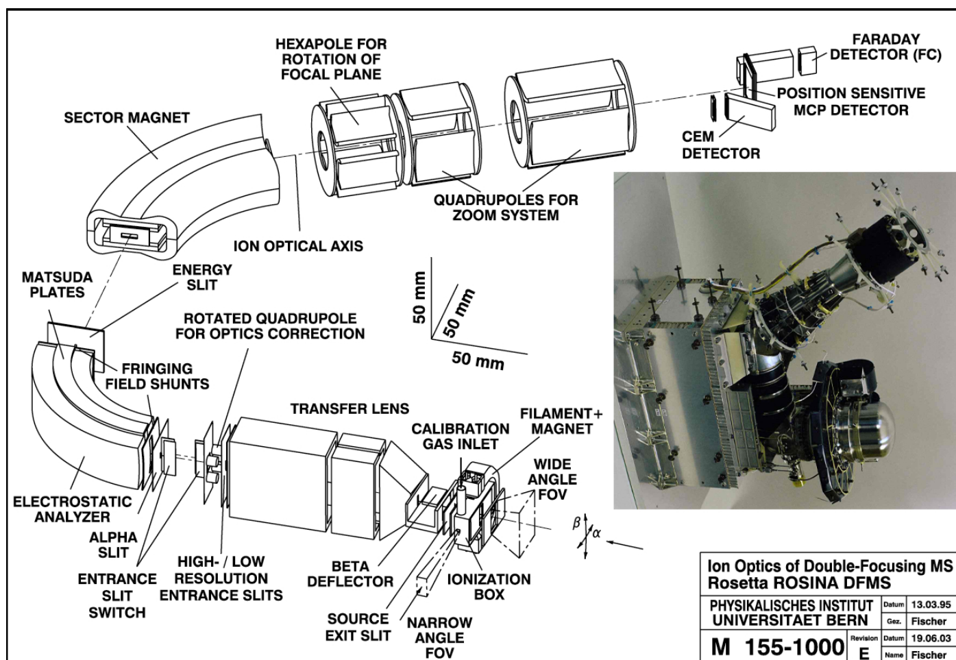
Fig. 2. DFMS ion optics: neutrals enter the source where they are ionized ( bottom center ) before they pass the electrostatic analyzer ( left bottom ), the magnet ( top left ), and then arrive at the detector ( top right ). Taken from Balsiger et al. (2007) . The inset shows a picture of the DFMS sensor in the same orientation.
