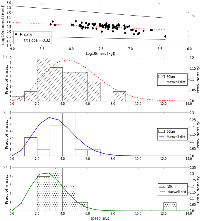
Fig. 9. a) Mass-dependent dust speed fitted to derive the power index \gamma = -0.32 \pm 0.18 ; b)–d) dust speed histograms and Maxwellian fits for particles detected at 30, 20, and 10 km, respectively. The error of the speed measurement is 6%.
