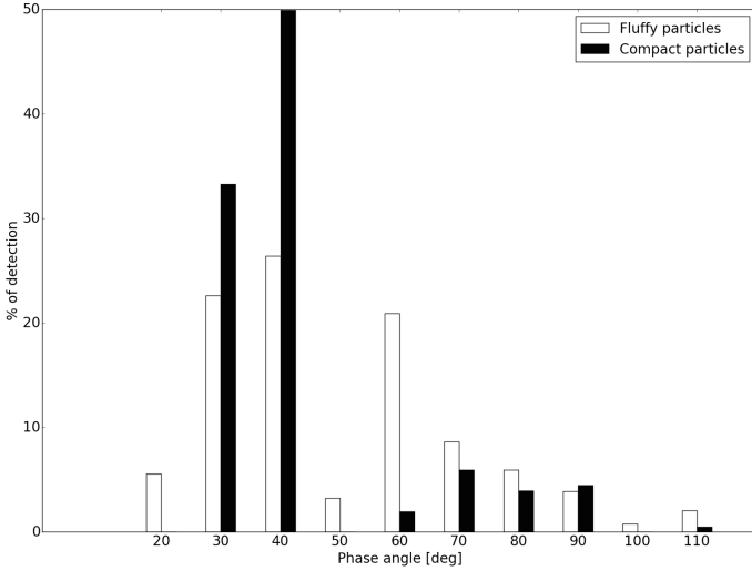
Fig. 5. Percentage of particles with respect to the phase angle at which they were detected. The particle numbers are doubly normalized: 1) the number of particles detected at each phase angle divided by the total number of particles of that specific type was calculated; and 2) the obtained ratio was normalized to the time spent by the spacecraft at specific phase angles.
