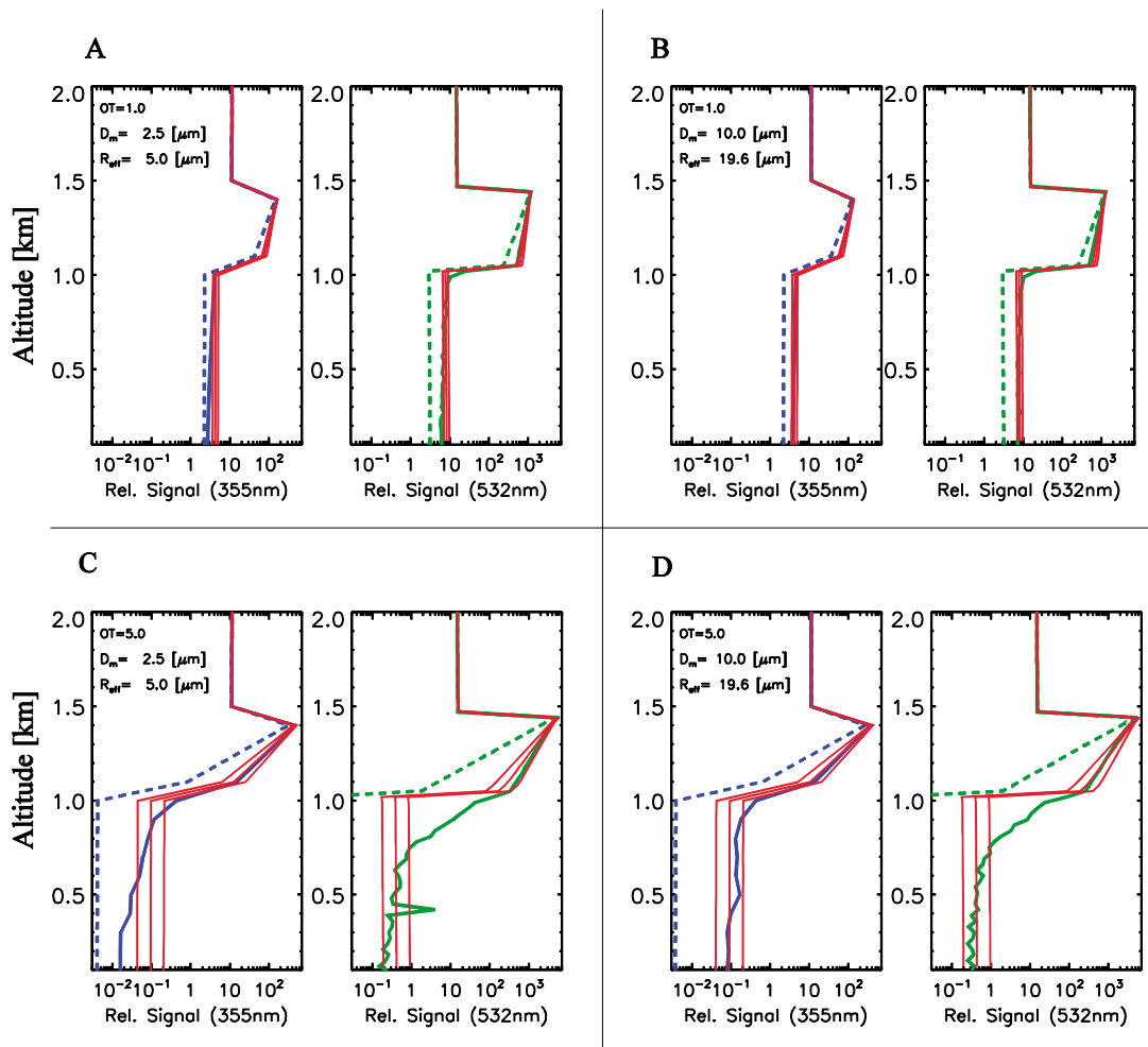
Figure B2. Example results of MC lidar radiative transfer simulations for AT Lidar (blue lines), CALIPSO (green lines) compared to the expected single-scatter signal levels for idealized water clouds (dotted Lines) and equation (A1) with \eta = 0.4, 0.5 , and 0.6 (red-Lines) for the CALIPSO simulations while \eta = 0.3, 0.4 , and 0.5 have been used for the AT Lidar simulations. The cloud optical thickness and particle sizes are as indicated in the plots. Spikes under the cloud are due to the statistical nature of the MC calculations and the small number of photon packets penetrating the cloud.
