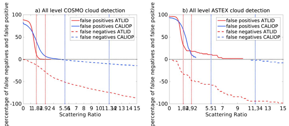
Figure C4. Percentage of false negatives cloud detections and false positives cloud detections as a function of the scattering ratio. The red (respectively blue) curve represents the ATLID detections (respectively CALIOP detections) for (a) COSMO case and (b) ASTEX case for different SR threshold values. Red vertical dotted lines represent the cloud day ( SR = 2.92 ) and night ( SR = 1.84 ) detection thresholds for ATLID. Blue vertical dotted lines represent the cloud day ( SR = 11.34 ) and night ( SR = 5.51 ) detection thresholds for CALIOP.
