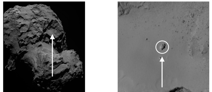
Fig. 7. Boulder-like feature in the Seth region. The center of this feature is the second of two additional secondary features for the zero-longitude definition of the Cheops reference frame. Context image ( left ): subset of NAC_2014-08-06T03.19.48.123Z_ID20_1397549900_F22. Close-up ( right ): subset of NAC_2014-08-28T18.42.56.579Z_ID20_1397549500_F22.
