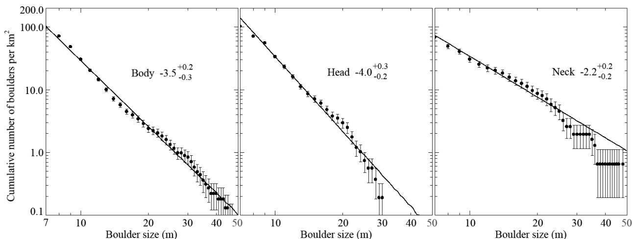
Fig. 10. Cumulative size-frequency distribution of \geq 7 m boulders per \text{km}^2 on the body, head, and neck.
