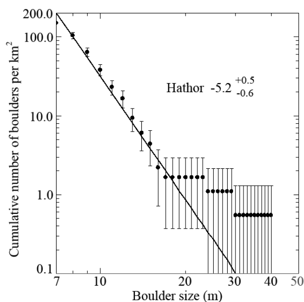
Fig. 12. Size-frequency distribution per \text{km}^2 on the Hathor fractured cliff. The poor statistics were enhanced by the 1 m binning for boulders larger than 18 m. These values cannot be considered in the fit, as explained in footnote 4.
