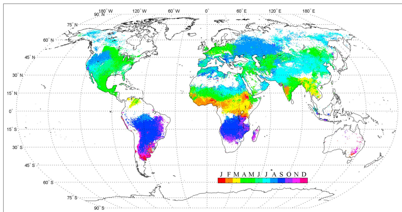
Figure 3. Month of maximum \text{NH}_3 column determined in 0.25^\circ \times 0.5^\circ cells from \text{NH}_3 measurements performed between 1 January 2008 and 31 December 2013. Monthly weighted columns associated with a weighted relative error above 35% have been set to zero.
