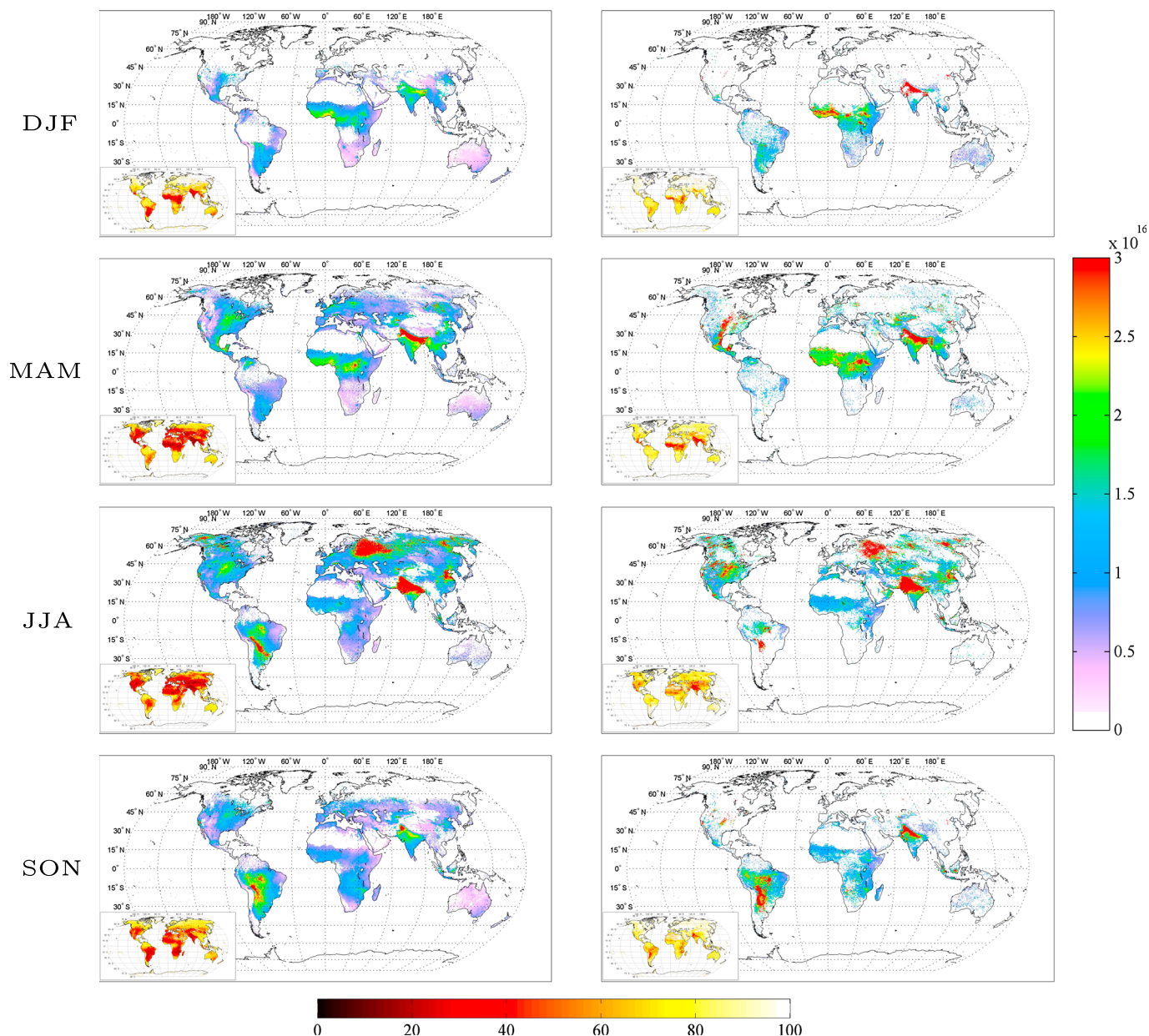
Figure 1. Composite seasonal distributions (molecules/cm 2 , vertical color bar) averaged over 6 years (1 January 2008 to 31 December 2013) of IASI-NH 3 (left column) morning and (right column) evening measurements in 0.25° × 0.5° cells. (first to fourth rows) December-January-February (DJF), March-April-May (MAM), June-July-August (JJA), and September-October-November (SON) weighted mean distributions. A postfiltering consisting in excluding mean column values associated with a mean relative error above 75% has been applied. Relative weighted error distributions (%; not filtered, horizontal color bar) are presented as an inset in the bottom left corner of each seasonal map.
