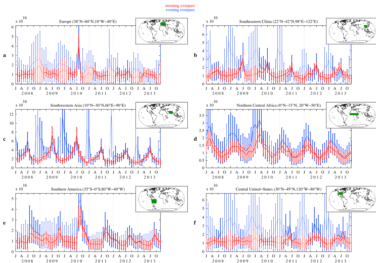
Figure 2. Monthly weighted time series of the \text{NH}_3 total columns ( \text{molecules}/\text{cm}^2 ) for the morning (red) and evening (blue) IASI overpasses covering the entire period from 1 January 2008 to 31 December 2013. Bold lines and error bars correspond to monthly means associated with a relative error below 75%. Each January is marked with a dashed vertical line, while the x axis labels are January (J), April (A), July (J), and October (O); the different years are also indicated on the time axis. The subcontinental areas selected are similar to the ones from Shephard et al. [2011] and are indicated by green patches in the upper right corner inset map.
