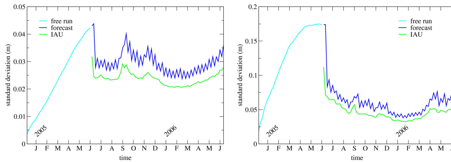
Figure 7. SSH time series of standard deviations for free-run, forecast and IAU ensembles over the Gulf Stream verification area (left panel) and the Z focus area (right panel).
