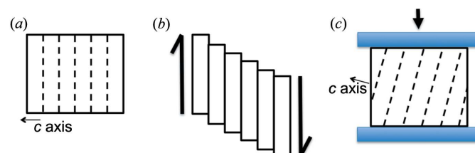
Figure 1 Schematic diagrams of (a) a single crystal of ice, (b) its directional deformation leading to glides in the basal plane and (c) the boundary conditions imposed by a rigid-blade displacement, which are not compatible with a homogeneous distribution of the basal glides.
