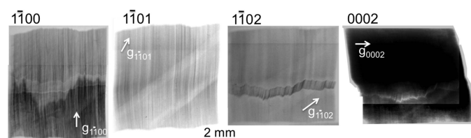
Figure 7 The variation in contrast of the grain sub-boundary for the 1\bar{1}00 , 1\bar{1}01 , 1\bar{1}02 and 0002 reflections after 7 h of loading. The oblique band (particularly visible on the 1\bar{1}01 image) corresponds to the absorption of the incident beam by the compressed-air pipe used for the loading.
