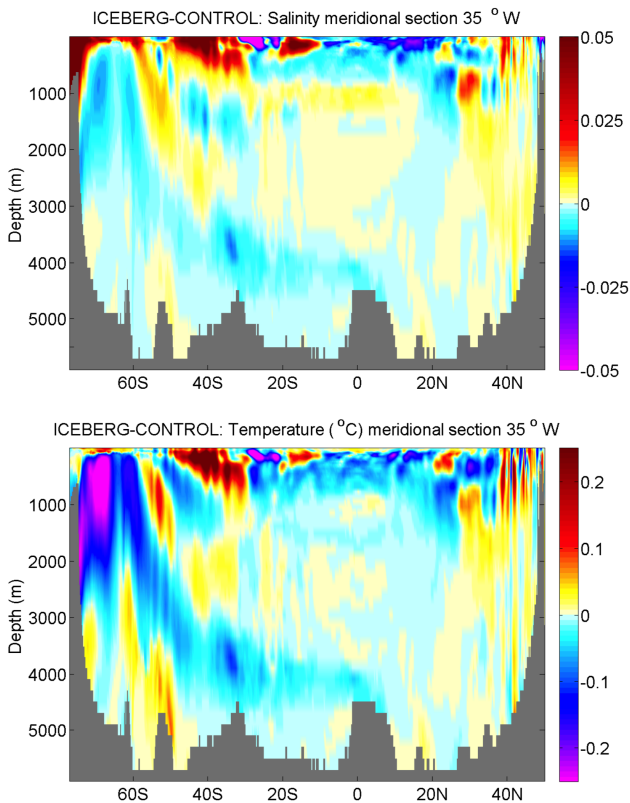
Figure 8. Meridional transect along 35° W, showing changes in salinity (upper panel) and temperature (lower panel), averaged over years 26–30.
