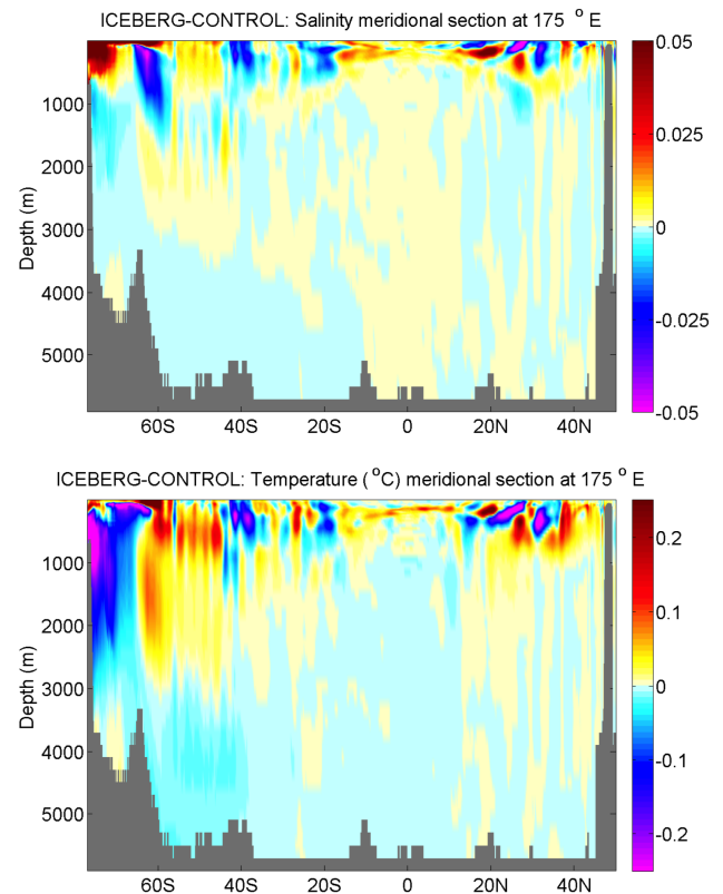
Figure 9. As Fig. 8, at 175° E.
