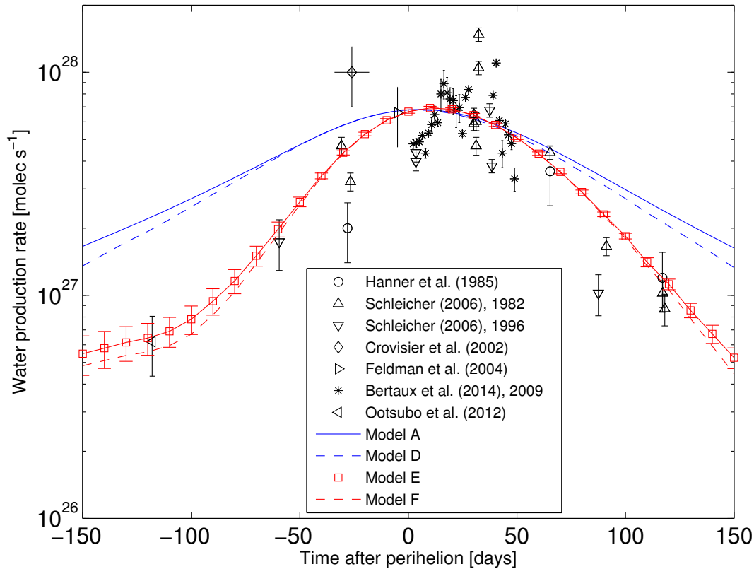
Fig. 18. Water production rates of comet 67P measured during earlier apparitions near perihelion. Models A and D for a homogeneous nucleus are scaled to the observed maximum. Model E is a best fit for spotted activity. Model F is calculated for the same distribution but with a thermal inertia of 100 \text{ [J m}^{-2} \text{ K}^{-1} \text{ s}^{-1/2}] .
