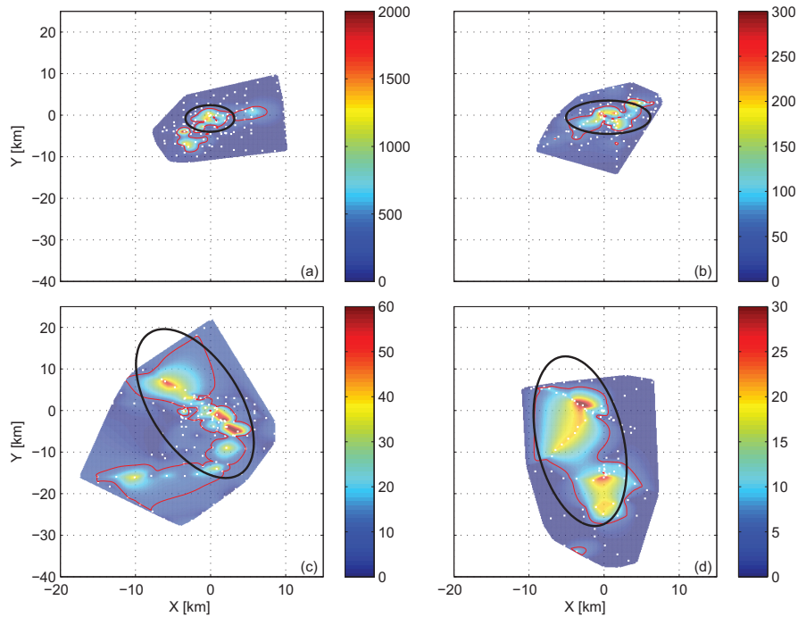
Figure 2: Lagrangian maps of SF_6 concentration [ f\text{mol L}^{-1} ] for Mapping 1 (a), Mapping 2 (b), Mapping 3 (c) and Mapping 4 (d). The plots are referenced to the position of the center mass. Note that the color bar maximum varies with each mapping. The [SF_6]_{max}e^{-2} contour lines are shown in red in each plot indicating the patch area with the contour line technique ( A_{CL} ). Gaussian ellipsoids are shown in black in each plot indicating the fitting patch area ( A_{GE} ). The locations of SF_6 measurements are indicated by the white dots.
