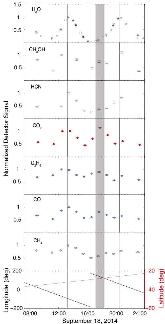
Fig. 2. Normalized intensity profiles of various volatiles for September 18, 2014. The error bars represent the ion statistical counting uncertainty, which is calculated as \sqrt{n} ( n is the number of ions detected), and in some cases, they are smaller than the symbol used (e.g., H_2O ). Vertical lines correspond to H_2O maxima. The shaded regions correspond to the CO_2 , C_2H_6 , and CO maxima independent of H_2O (see text). Bottom panel: Sub-spacecraft longitude and latitude as a function of time (UT). Data gaps are due to reaction wheel offloading. The distance of Rosetta from the comet nucleus was 28.6 km, and the heliocentric distance on this date was 3.34 AU.
