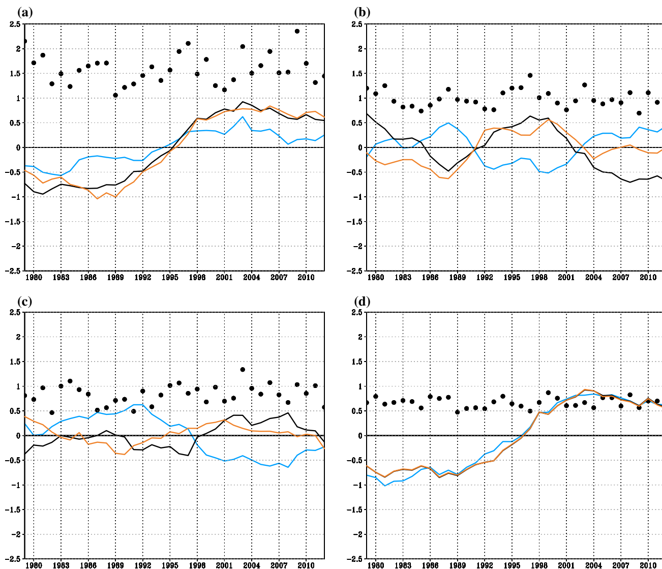
Fig. 4 Temporal evolution of the standardized quantile 10 ( blue lines ), quantile 90 ( red lines ) and of the median of the SHL intensity ( black lines ) for each year from 1979 to 2012 using the unfiltered
