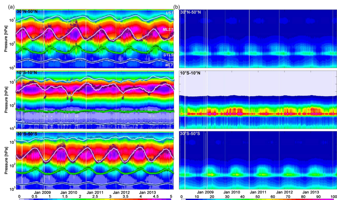
Figure 4. (a) Daily IASI \text{O}_3 profiles ( 1 \times 10^{12} molecules \text{cm}^{-3} ) for the period 2008–2013 and over the range of the retrieved profiles as a function of time and altitude, in three latitude bands: 30–50° N (top), 10° S–10° N (middle) and 30–50° S (bottom). Superimposed daily IASI \text{O}_3 partial columns (scatters) and the associated fits (solid lines) from the multivariate regressions for the MLT (ground–300 hPa), UTLS (300–150 hPa), MLST (150–25 hPa) and UST (above 25 hPa) layers. The IASI measurements and the fits have been scaled for clarity. (b) Estimated total retrieval errors (%) associated with daily IASI \text{O}_3 profiles.
