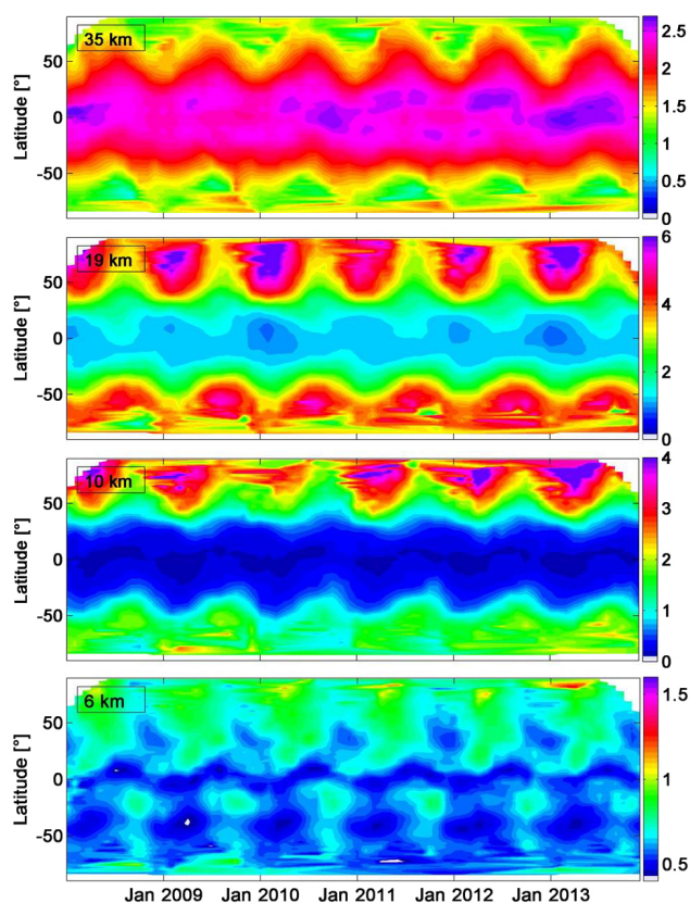
Figure 6. Daily IASI O 3 number density ( 1 \times 10^{12} molecules \text{cm}^{-3} ) at 35 km (top row), 19 km (second row), 10 km (third row) and 6 km (bottom row) as a function of time and latitude. Note that the colour scales are different.
