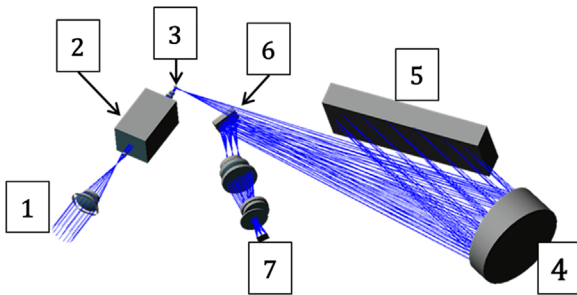
Fig. 2. Schematics of the SO and LNO channels: (1) the entrance optics, (2) the AOTF filter, (3) the spectrometer entrance slit, (4 and 6) folding mirrors, (5) the echelle grating, (7) the detector.
