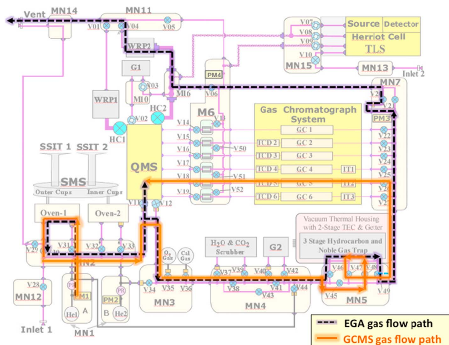
Figure 3. The SAM gas flow diagram showing the helium gas flow paths in both EGA (purple dashed line) and GCMS modes (orange line). Major components shown include the quadrupole mass spectrometer (QMS), the gas chromatograph system including six columns (GCx), three injection traps (ITx), and five thermal conductivity detectors (TCDx), the tunable laser spectrometer (TLS), the gas manifolds (MNx), the microvalves (Vx) and high-conductance valves (HCx), the hydrocarbon and noble gas trap, the sample manipulation system (SMS) with two solid sample inlet tubes (SSIT-1 and SSIT-2) and two pyrolysis ovens (Oven-1 and Oven-2), the helium gas reservoirs (He-1 and He-2), pressure sensors (PMx), and miniature wide-range pumps (WRP-1 and WRP-2). The manifold and pipe heaters and associated temperature sensors are not shown.
