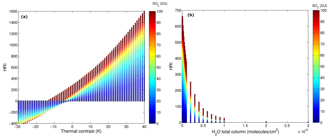
Figure 2. Example of interpolated LUT to convert HRI in SO 2 column depending on thermal contrast and water vapour for the angle bin 15–20°. The colour bar represents the 0–4 km column of SO 2 in DU. Panel (a) shows the dependency of HRI on thermal contrast (constant total column of H 2 O of 2 \times 10^{20} molecules cm -2 ); panel (b) shows the dependency on the total column of water (constant thermal contrast of 15 K).
