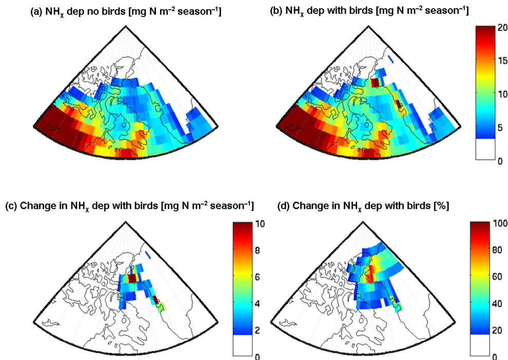
Figure 8. GEOS-Chem simulation of total NH x deposition (in mg N m -2 season -1 ) for the months May to September (inclusive). Panel (a) does not include seabird emissions, whereas the panel (b) does. The difference in total NH x deposition between the two emissions scenarios (with birds minus without birds) is shown in panels (c) and (d) as an absolute amount and percentage increase, respectively.
