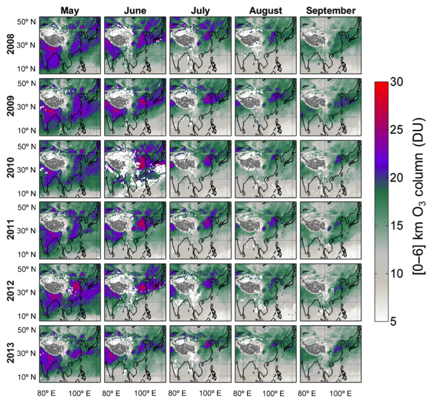
Figure 1. Monthly averaged daytime tropospheric 0–6 km O_3 column from IASI over the EASM region and period (May–September) for the years 2008–2013. The decrease due to the monsoon is more prominent to the south of the domain.
