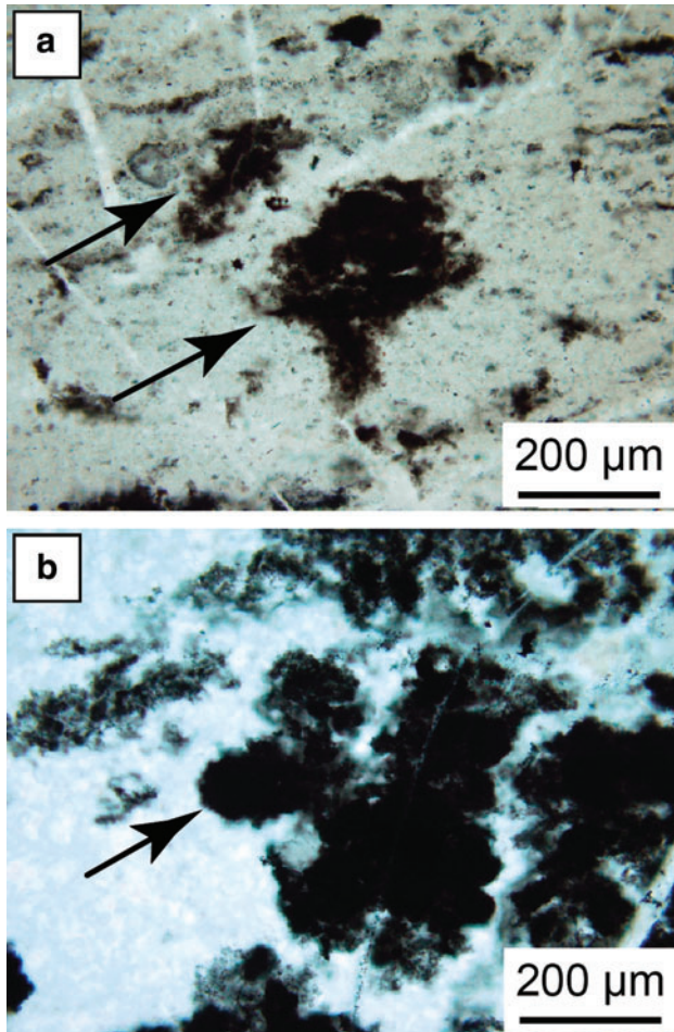
FIG. 8. Light micrographs of “free-floating” clots. (a) Clots (arrows) characterized by irregular shapes and spiky protuberances that apparently developed in situ in strongly hydrothermally influenced sediments (same facies as in Fig. 7a). Faint wisps of carbon outline the very fine-grained sediment beds. (b) Clot (arrow) with an irregular but slightly more rounded shape, developed in primary hydrothermal silica. (Color graphics available at www.liebertonline.com/ast )
