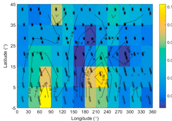
Figure 2. Scaled density at 130 km binned by latitude and longitude, with crosses showing the location of the individual profiles. Observations are made between 1340 and 1500 LST at L s = 217°–219°. A value of 0.1 (km -1 ) corresponds to a density of ~10 11 cm -3 assuming σ ~ 10 -17 cm 2 .
