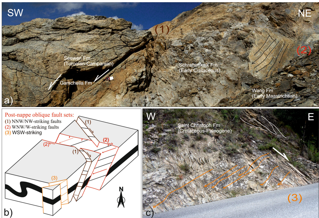
Fig. 6 Cross-cutting fault relationships. a Fault set (1) is cross-cut by (2), with the main slickenshire direction on this plane indicated by thin black lines with arrowheads. Wildstrubelhütte, (602508/136659). For scale, a square bright compass can be seen immediately below the white arrow of fault set (1). b Schematic block diagram, showing the distinction between the three post-nappe oblique fault sets (1), (2) and
