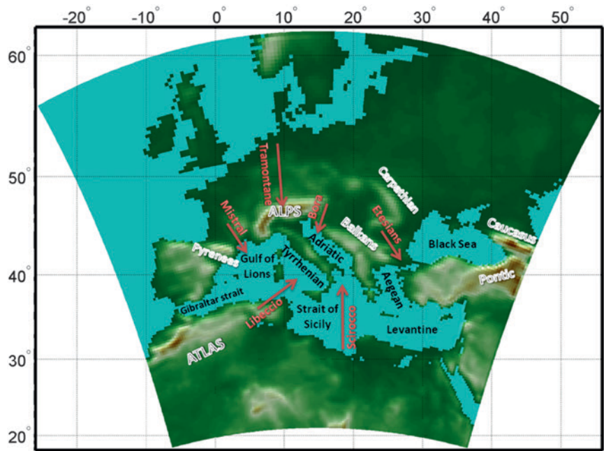
FIG. 1. Maximum model integration area for coupled systems.
