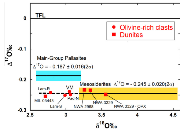
Fig. 6. Oxygen isotope composition of olivine-rich clasts in mesosiderites compared to main-group pallasites (this study) and other mesosiderite samples ( Greenwood et al., 2006 ). Shaded zones show the \pm 2\sigma variation on group mean values. Lam = Lamont, VM = Vaca Muerta, Pad = Mount Padbury. TFL = terrestrial fractionation line. Analysis of MIL 03443 from Greenwood et al. (2014) .
