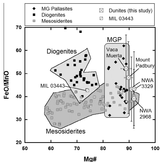
Fig. 4. The composition of olivine from mesosiderite olivine-rich clasts and related dunites (NWA 2968, NWA 3329) compared to main-group pallasites, mesosiderites and diogenites. Error bars 2\sigma . Main Group Pallasite (MGP) data: Mittlefehldt, 1980 ; Mittlefehldt et al., 1998 ; Boesenberg et al., 2012 . Diogenite data: Sack et al., 1991 ; Mittlefehldt et al., 1998 ; Mittlefehldt, 2000 ; Irving et al., 2003 ; Barrat et al., 2006 ; Beck and McSween, 2010 ; Scheerer et al., 2010 . Mesosiderite data: Delaney et al., 1980 ; Mittlefehldt, 1980 ; Prinz et al., 1980 ; Mittlefehldt et al., 1998 ; Terribilini et al., 2000 ; Kong et al., 2008 . Note: olivine in mesosiderites occurs as small grains in the matrix and as coarse cm-sized grains and dunitic clasts. The data of Mittlefehldt (1980) was exclusively from these larger grains. In comparison, the largest dataset plotted in Fig. 4 is from Delaney et al. (1980) , which includes analyses from all mesosiderite olivine types. The large coarse-grained olivines and the smaller matrix types are likely to be from different sources.
