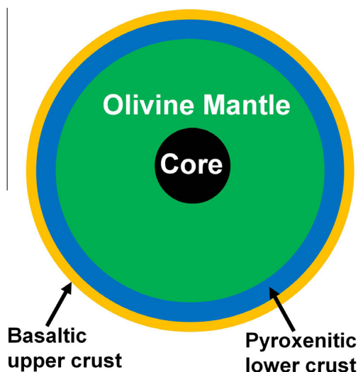
Fig. 1. Schematic cross-section of the interior of a hypothetical differentiated asteroid formed as a result of melting of a chondritic starting composition. The exact thickness of the individual layers calculated by modelling studies (Ruzicka et al., 1997; Righter and Drake, 1997; Mandler and Elkins-Tanton, 2013; Toplis et al., 2013) is dependent on the assumed starting composition.
