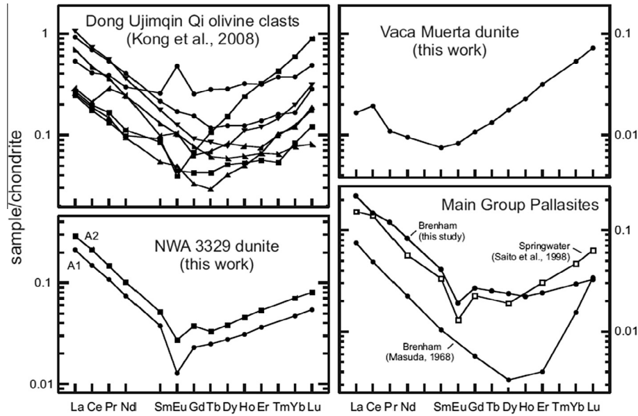
Fig. 7. CI normalized Rare Earth Element plot for the Vaca Muerta and NWA 3329 dunitic clasts compared to that of olivine clasts from the Dong Ujimqin Qi mesosiderite Kong et al. (2008) , and olivine from the Brenham and Springwater pallasites ( Masuda, 1968 ; Saito et al., 1998 ; this study).
