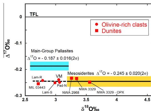
Fig. 6. Oxygen isotope composition of olivine-rich clasts in mesosiderites compared to main-group pallasites (this study) and other mesosiderite samples ( Greenwood et al., 2006 ). Shaded zones show the \pm 2\sigma variation on group mean values. Lam = Lamont, VM = Vaca Muerta, Pad = Mount Padbury. TFL = terrestrial fractionation line. Analysis of MIL 03443 from Greenwood et al. (2014) .
