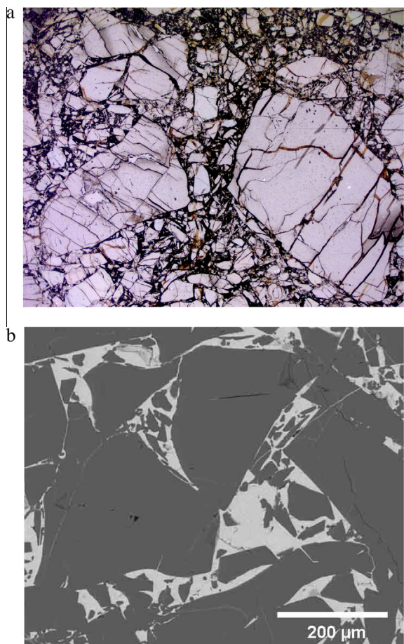
Fig. 2. Vaca Muerta dunite clast. (a) (top). The Vaca Muerta clast consists of cataclastic textured olivines in a dark matrix. (plane polarized light. Field of view 7 mm). (b) (bottom). Backscattered electron image of the Vaca Muerta clast showing that the angular olivine fragments are enclosed in a sulfide-rich matrix.
