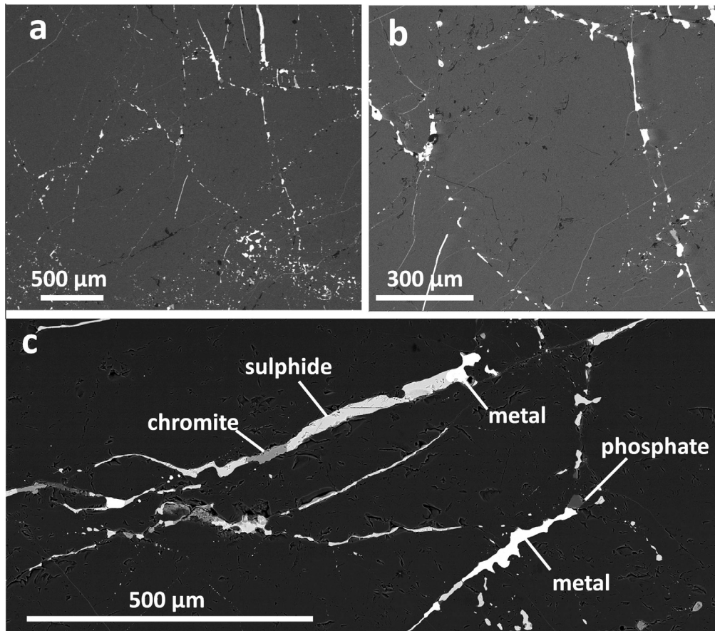
Fig. 3. Backscattered electron images of Mount Padbury inclusion “N”. (a) (top left): Large centimetre-sized olivines McCall (1966) are traversed by a network of thin veinlets mainly composed of iron sulfide with accessory chromite, phosphate and Fe,Ni metal. Note that not all fractures are completely occupied by accessory phases. (b) (top right): Higher magnification image of the central area of (a) showing thin (10–30 \mu\text{m} ) veinlets and blebs of iron sulfide along the margin of angular olivine grains. (c) (bottom): detail of area in the top central part of (a). Olivine is essentially unzoned and traversed by fracture sets filled by sulfide, metal, chromite and phosphates.
