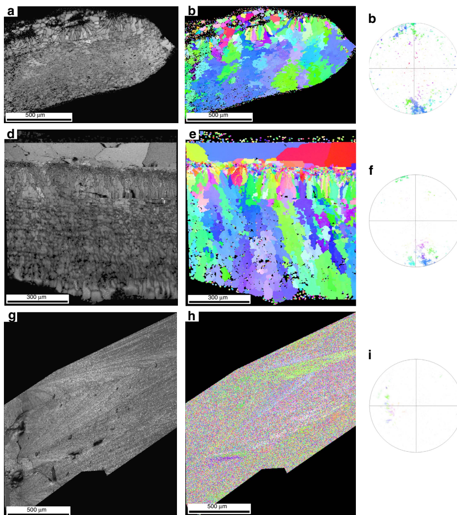
Figure 5 | EBSD analysis of Mongolian and French eggshells. Images are representative of multiple specimens examined. Colour coding is as described in Fig. 4. (a–c, d–f) Two different individual Mongolian Oviraptorid eggshells, respectively. Both eggshells show an overall good preservation, with no evidence for recrystallization and calcite crystals displaying a preferred crystallographic orientation of the c axis perpendicular to the shell exterior, as shown in pole figures. In this respect, data are similar to Auca Mahuevo layer-4 eggshells in Fig. 4. There are some indications of deformation of calcite crystals, possibly due to eggshells being compressed on burial, as indicated discontinuity and deformation of crystal boundaries as seen in diffraction maps and a larger spreading of poles on the projection of the {0001} plane of calcite than typically observed in modern eggshells. For comparison, the bottom panels (g–i) show data from a Rousset level-A eggshell that is completely altered and recrystallized, with none of the original microstructure typical of eggshells observed. Instead, the eggshell has been replaced by microcrystalline calcite with low diffraction, and the pole figure (i) shows the absence of biological control over crystallographic orientation.
