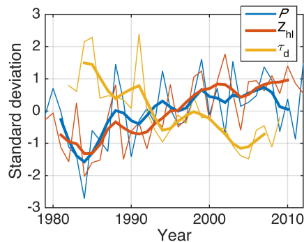
Upper: Seasonal (June-August) time series of Zhl (red), precipitation ( P , blue) and td (yellow). The monthly mean precipitation series is averaged over 5° W to 20° E, 10° to 20° N, and td is averaged over 10° to 65° W and 0° to 30° N. The thin lines are the seasonal means and the thick lines are the 5-season smoothed time series (via a 1-4-7-4-1 filter).
