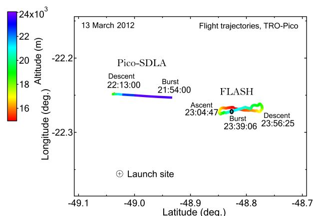
Figure 3. Balloon trajectories of Pico-SDLA and FLASH flights on 13 March 2012. The trajectories are color-coded with altitude. The time is given in UTC. The ascent and descent time stamps correspond to times when the balloon passed an altitude of 15 km. The burst altitude is localized using a “○” marker.
