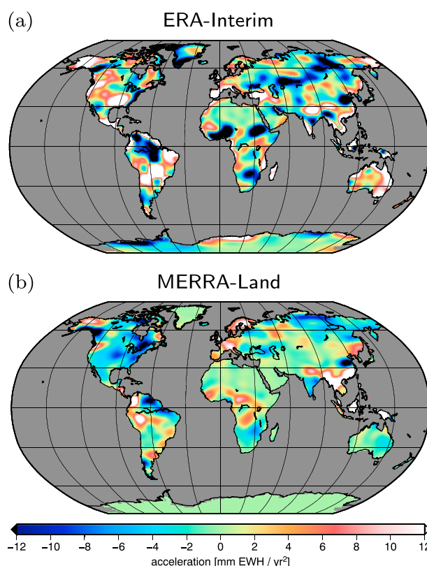
Figure 2. Average acceleration of water storage (EWH = equivalent water height) from reanalyses for the time span 2003–2012.
