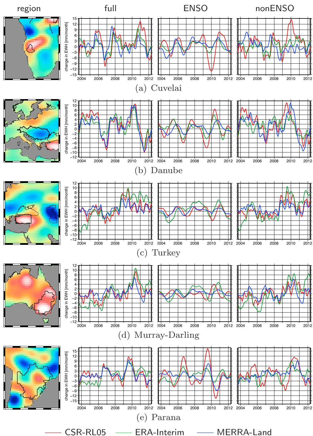
Figure 6. Time series of water fluxes for different regions. The first column shows the region border and the acceleration signal as seen by GRACE (representing a zoom in from Figure 1b). The time series represent the full signal (second column), the ENSO mode (third column), and the non-ENSO mode (fourth column).
