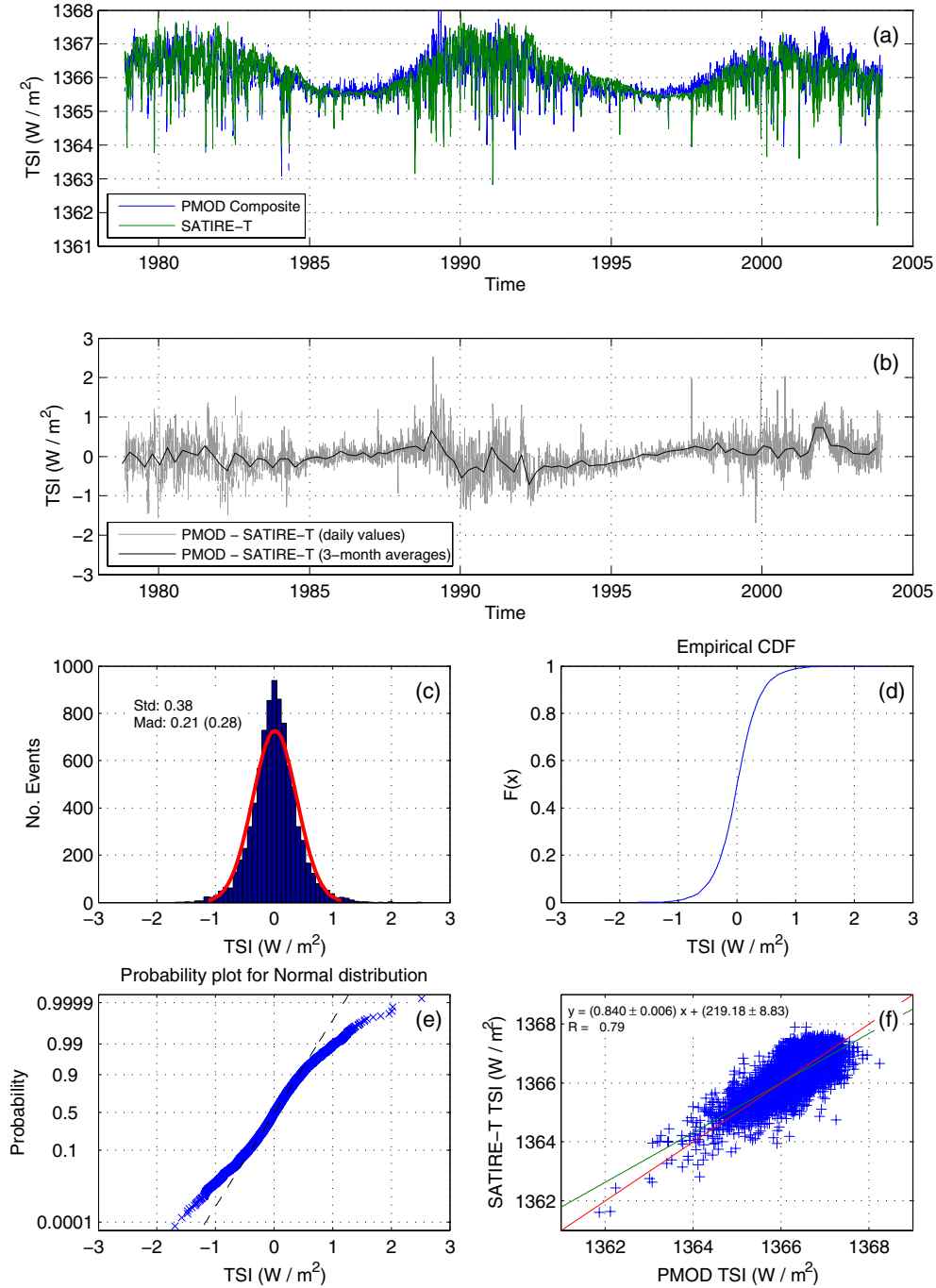
Fig. 2. a) Comparison between the observed (PMOD Composite; blue line) and the modeled (SATIRE-T; green line) TSI from Nov./1978 to Dec./2003. b) Difference between the observed and modeled TSI. The gray and black lines present the daily and 90-day averaged values, respectively. c) Distribution of the difference between daily values of the observed and modeled TSI (model error). The standard deviation and the median absolute deviation are indicated in the panel. The red curve represents the corresponding probability distribution function for the normal distribution with the mean and standard deviation of the model error. d) Cumulative distribution function (CDF) for the difference between observed and modeled TSI. e) Probability plot for normal distribution with the mean and standard deviation of the model error. f) Scatter plot of the observed versus modeled TSI. The red line indicates the set of expectation values of the model. The correlation coefficient and the coefficients of the best linear fitting (green line) are presented in the panel. The p -value for testing the hypothesis of no correlation is lower than 0.5, which indicates that the correlation is significant.
