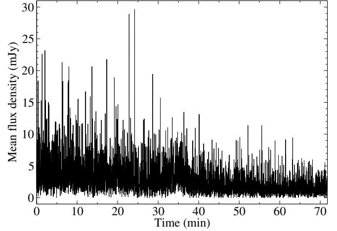
Fig. 1. Calibrated time series from PSR B0329+54. The decrease of the signal strength due to the weak interstellar scintillation is clearly visible.
