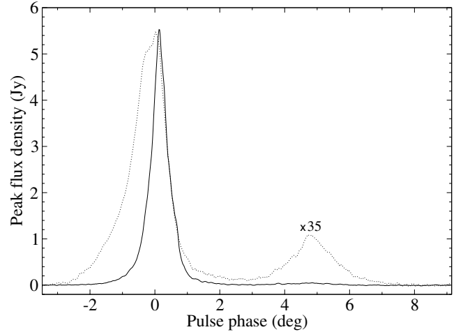
Fig. 7. Average profile (solid line) made by folding strong pulses from observations of PSR B1133+16 in April 2004 relative to the integrated profile (dotted line), multiplied by a factor of 35. The tendency of the strong single pulses to occur at the trailing edge of the first component can be seen.
