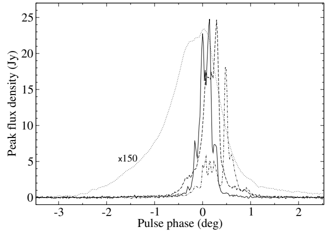
Fig. 8. Three strongest pulses (solid, dashed and dot-dashed lines) from observations of PSR B1133+16 in April 2004 relative to the first component of the integrated profile (dotted line), multiplied by a factor of 150. The complex pulse structure and tendency to occur at the trailing edge of the first component is shown.
