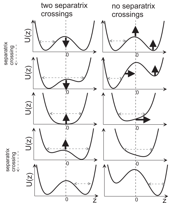
Fig. 6. Left column shows successive profiles of U(z) and particle positions (from top to bottom) for transition from left well to right well with two separatrix crossings. Right column shows the same transition, but without separatrix crossings. Grey arrows correspond to particle position U = 1/2 and black arrows show direction of U(z) deformation.
