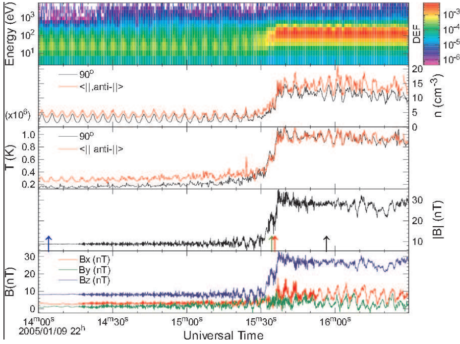
Fig. 20 Overview of data from Cluster 2 on 2005 Jan 9. From top to bottom: Omni-directional electron energy-time spectrogram @ 250 ms resolution, electron pseudo-density, electron pseudo-temperatures (see Method), magnetic field magnitude, and field components. Arrows in the fourth panel show locations of the cuts presented in Figure 22. (Adapted from Schwartz et al. 2011).
