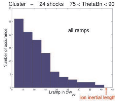
Fig. 6 Histogram of the 96 shock ramp thicknesses. Reprinted with permission from (Mazelle et al. 2010). Copyright 2010, American Institute of Physics.
