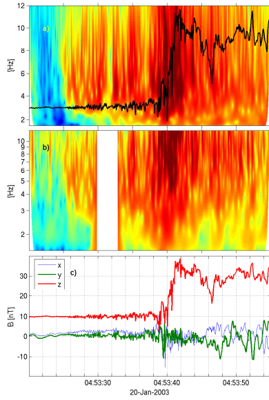
Fig. 15 Magnetic and electric fields in the Normal Incidence Frame (NIF) of a high Mach number shock. a) Power spectra of the magnetic field (STAFF). The black line is the DC total magnetic field, included to show the waves in relation to the shock ramp structure. b) Power spectra of the electric field (EFW). The data gap is due to instrumental interference. c) The magnetic field in NIF coordinates B_{\text{NIF}} . (Adapted from Sundkvist et al. 2012)
