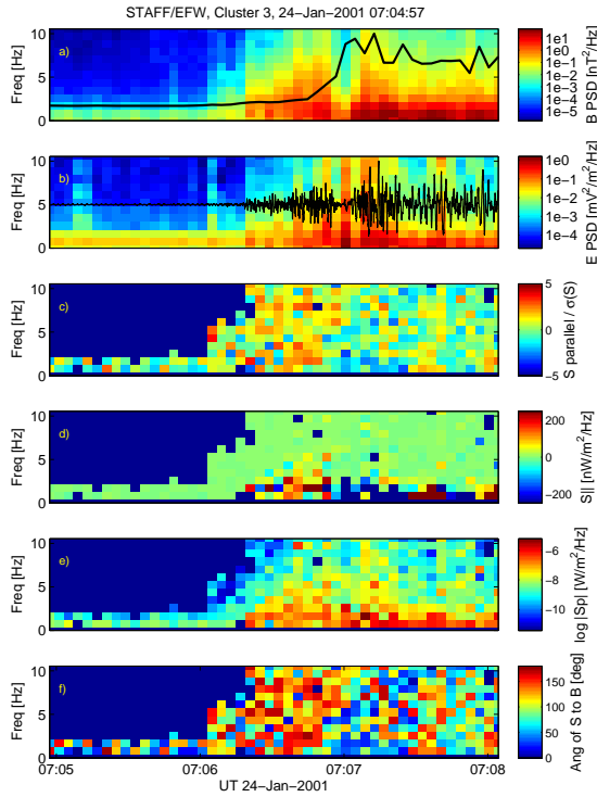
Fig. 18 Poynting flux derived from electric and magnetic fields for a high Mach number shock. a) Wave magnetic field and averaged B_0 . b) Wave electric field. c) S_{\parallel} normalized by its standard deviation (yellow and red corresponds to upstream flux). d) S_{\parallel} . e) \log_{10} S_{\parallel} . f) Angle of S to \mathbf{B}_0 (red meaning upstream). (Adapted from Sundkvist et al. 2012)
