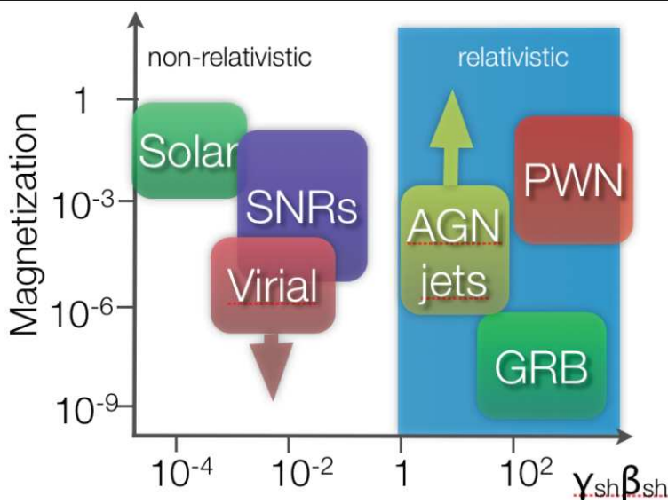
Fig. 1 (courtesy of A. Spitkovsky). Parametric range of observations of collisionless shocks associated with different astrophysical objects.
