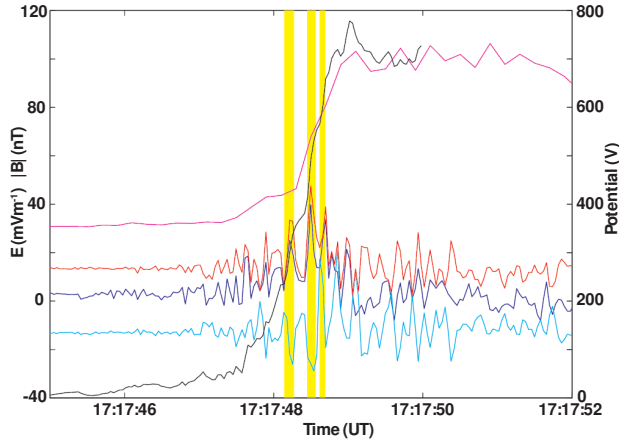
Fig. 9 The FGM magnetic and EFW electric fields measured by Cluster 1 on March 31 st , 2001 around 17:18 UT. The magnetic field magnitude is shown by the magenta line. The spin plane electric field magnitude, and E_x and E_y components are shown in red, blue and cyan respectively. The yellow regions highlight the periods when large amplitude short duration spikes in the electric field are observed. The black line (Y scale of RHS) represents the change in potential within the shock. (Adapted from Walker et al. 2004)
