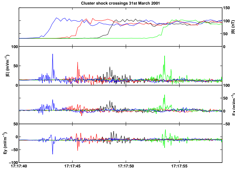
Fig. 8 Overview of the shock crossing on March 31 st , 2001 at 1718 UT. The top panel shows the magnitude of the magnetic field measured by FGM. The second panel shows the magnitude of the electric field measured in the satellites spin plane. The lower two panels show the spin plane components E_x and E_y . (Adapted from Walker et al. 2004)
