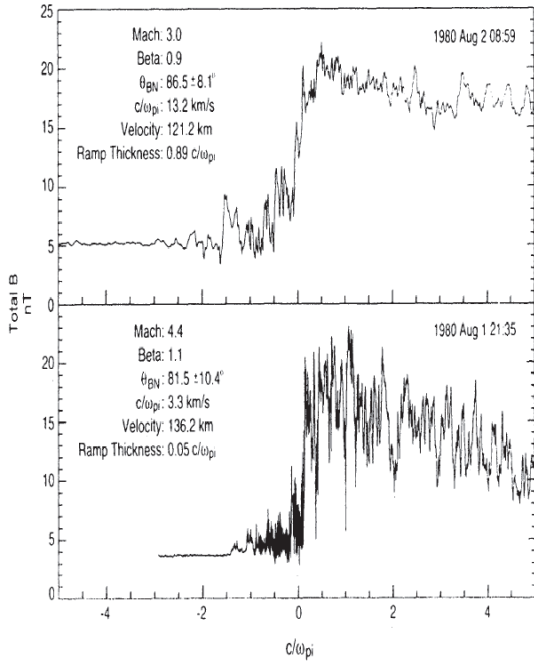
Fig. 3 These shocks formed under similar solar wind conditions, but there is great disparity between their ramp widths (Adapted from Newbury and Russell 1996).
