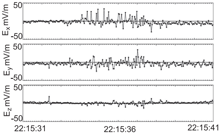
Fig. 23 Electric field measured onboard Cluster 2 satellite from 22:15:31 to 22:15:41. Electric field bursty spikes having amplitudes of 20\text{-}40\text{mVm}^{-1} having duration of the order of 0.1 sec are clearly seen during ramp crossing. Figure is provided by F. Mozer.
