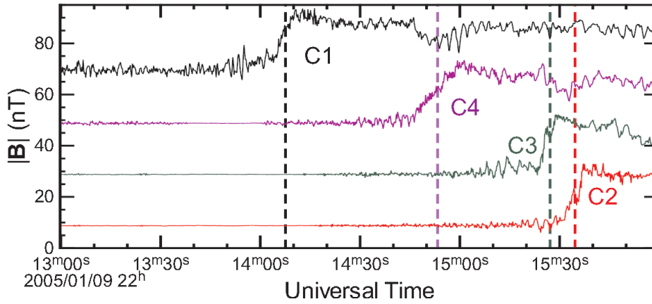
Fig. 19 Magnetic field data at a crossing of the Earth's bow shock by the 4 Cluster spacecraft on 9 Jan. 2005. Traces have been shifted by 20 nT for clarity. The dashed lines show the times of the steep ramp. (Adapted from Schwartz et al. 2011).
