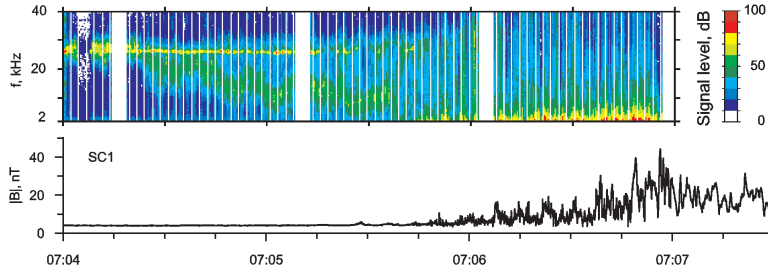
Fig. 32 (top) Electric field spectra and (bottom) magnetic field profile obtained during the Earth's bow shock crossing on 24 January 2001 aboard SC1. The frequency-time spectrogram is measured by the Whisper experiment. The vertical white bands correspond to the time intervals when no data were obtained in the natural wave mode. The wave intensity is colour coded with the reference level of 10^{-7} V_{rms}/\text{Hz}^{1/2} , where rms is the root mean square to notify the averaged level of the fluctuating electric field variance. The magnetic field profile is obtained by FGM experiment. The time scales for the both panels are the same. (Adapted from Lobzin et al. 2007).
