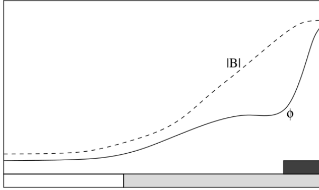
Fig. 7 Sketch of the changes observed in the magnetic field and electrostatic potential during the crossing of a quasi-perpendicular shock (based upon the experimental results of (Eselevich et al. 1971))
