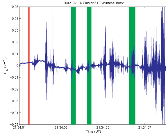
Fig. 25 Waveforms of electric field measurements during shock front crossing on February 26 th , 2002 at 2134 UT. The vertical lines mark periods where the waves were registered. As it will be shown later red vertical lines mark periods where the waves were identified as ion-sound, two first green columns as lower-hybrid electrostatic waves, third green column as whistler waves in lower hybrid frequency range.
