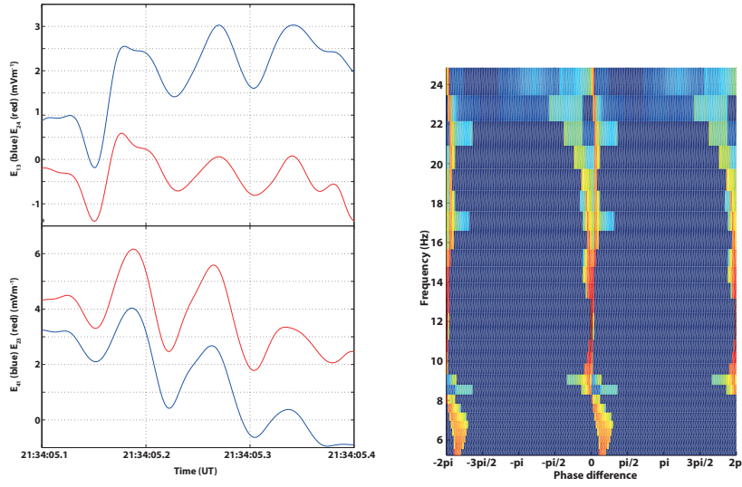
Fig. 29 Panel(1): The \omega - k joint spectrum calculated from the phase differences measured between the two parallel electric field components E_{13} and E_{42} for event 1. Panel (2): The electric field waveforms E_{13} and E_{42} (top panel) and E_{41} and E_{23} (lower panel) for the first event. (Adapted from Walker et al. 2008).
