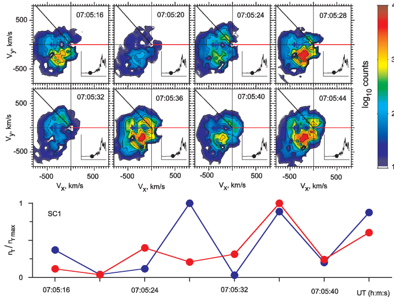
Fig. 33 (top) Ion velocity distributions obtained from CIS measurements within the forward part of the foot for the Earth's bow shock crossing on 24 January 2001 aboard SC1 and (bottom) temporal variations for the relative number of counts corresponding to reflected ions. The distributions were calculated in the GSE coordinates. In the bottom panel, a blue line corresponds to ions with V_y < 0 , while a red line shows the data for V_y > 0 . Strong variations of n_r , especially for V_y < 0 , show that the reflection of ions is bursty. The relative positions where the measurements were made are indicated by the dots on the magnetic field profiles shown as inserts. (Adapted from Lobzin et al. 2007).
