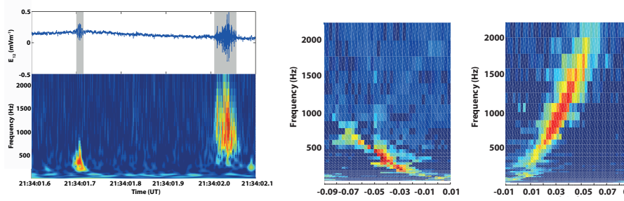
Fig. 26 Left: The waveform (top panel) and wavelet spectrogram (bottom panel) of the electric field computed from the difference in potential between probes 3 and 1. Centre and right: Examples of the f-k spectrograms for the first (left) and second (right) wave packets. (Adapted from Balikhin et al. 2005)
