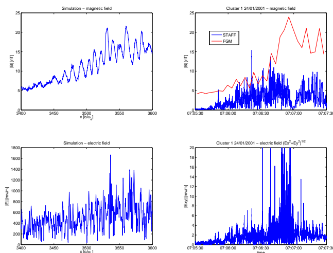
Fig. 34 Comparison of electric and magnetic fields observed on 24th of January 2001 by Cluster satellites and obtained in computer simulation by Comișel et al. (2011). Both panels show the fields in the vicinity of the foot/ramp regions. Top panels represent magnetic fields as measured by FGM instrument and STAFF search coil magnetometer (right), and obtained as a result of simulations(left). Bottom panels represent measured and simulated electric fields. One can see huge difference in amplitude of electric fields between measurements and simulations that results from artificial ratio of plasma to gyrofrequency and consequently unrealistic refractive index of waves. (Figure is provided by J. Soucek and H. Comișel)
