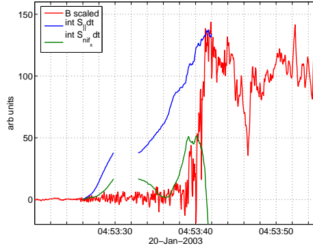
Fig. 17 Poynting flux integrated along the spacecraft trajectory. The blue line is a projection along the ambient magnetic field \int S_{\parallel} dt and the green line is a projection on the shock normal \int \mathbf{S} \cdot \hat{\mathbf{n}} dt . The red line shows the scaled magnetic field B_0 for reference. (Adapted from Sundkvist et al. 2012)
