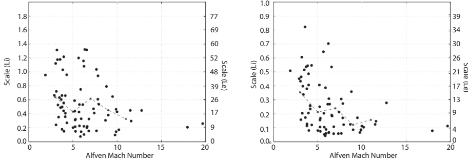
Fig. 4 Scatterplot of experimentally derived shock size (left panel) and shock spatial scale (right panel) normalized to the ion inertial scale length c/\omega_{pi} (left axis) and electron inertial scale c/\omega_{pe} (right axis) as a function of Alfvén Mach number. The dashed line represents the averaged values of shock width averaged over shocks with Alfvén Mach number in the ranges 2–4, 4–6, 6–8, 8–10, 10–12. The vertical lines represent the statistical error bars for each of these Mach number ranges. (Adapted from Hobara et al. 2010)
