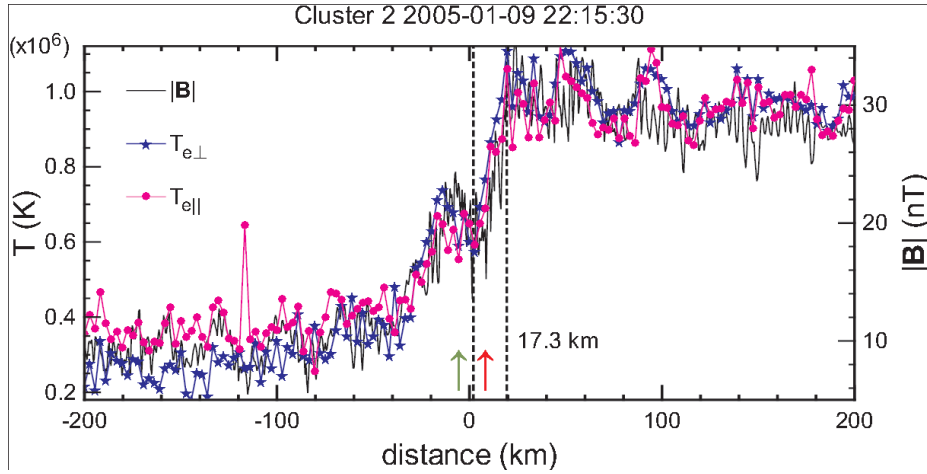
Fig. 21 Magnetic field (solid) and electron temperature (symbols) as a function of distance from the shock ramp. Roughly half the temperature rise occurs within the region 17.3 km wide between the dashed vertical lines corresponding to 6.4 electron inertial lengths ( c/\omega_{pe} ). (Adapted from Schwartz et al. 2011).
