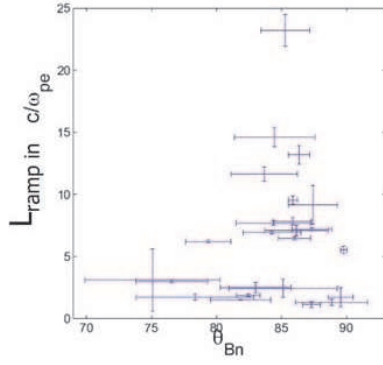
Fig. 5 Thinnest ramps observed versus shock \theta_{Bn} . Reprinted with permission from (Mazelle et al. 2010). Copyright 2010, American Institute of Physics.
