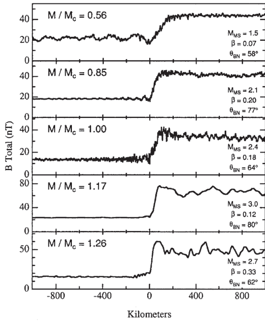
Fig. 2 The total magnetic field strength as a function of distance through five low beta, quasi-perpendicular shocks in order of increasing ratio of criticality. The Mach number, \beta , and \theta_{BN} for each shock are displayed. The data are shown at the highest temporal resolution available. The sampling rate for the first three shocks is 16 Hz and 4Hz for the last two (Adapted from Farris et al. 1993).
