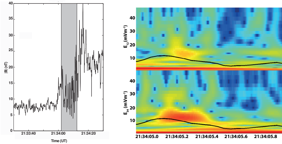
Fig. 28 Panel(1): The magnetic profile of the bow shock crossing observed by Cluster 3 on February 26 th , 2002 just after 2134UT. The period for which EFW internal burst mode data is available is indicated by the shaded region. Panel(2): The wavelet dynamic spectrogram of electric fields E_{12} (top) and E_{34} showing a the occurrence of oscillations just above the lower-hybrid resonance frequency (black line) for event 1. (Adapted from Walker et al. 2008).
