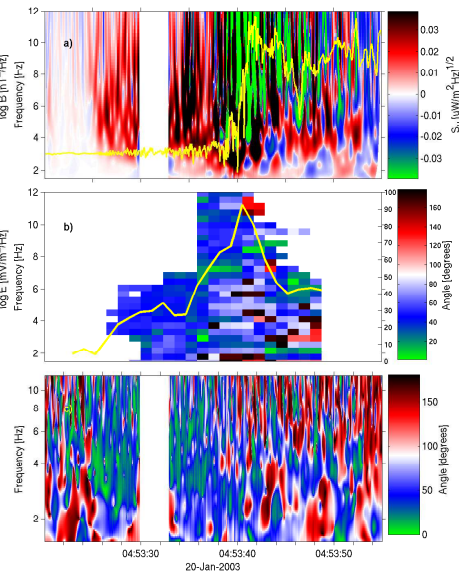
Fig. 16 Poynting flux in the Normal Incidence Frame (NIF) of the same shock as in Figure (15). a) Poynting flux S_{\parallel} projected on the local \mathbf{B}_0 in the NIF, where red corresponds to the upstream flux away from the shock. b) Angle \theta_{k,B} between \hat{\mathbf{k}} and magnetic field \mathbf{B}_0 . The yellow line represents the average over all frequencies (right scale). c) Angle between Poynting flux \mathbf{S} and \mathbf{B}_0 . (Adapted from Sundkvist et al. 2012)
