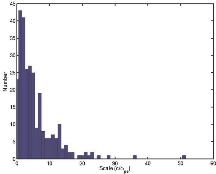
Fig. 10 Histogram of the scale sizes for the spike-like enhancements observed during a number of crossings of the quasi-perpendicular bow shock. (Adapted from Walker et al. 2004)
