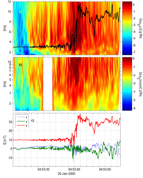
Fig. 15 Magnetic and electric fields in the Normal Incidence Frame (NIF) of a high Mach number shock. a) Power spectra of the magnetic field (STAFF). The black line is the DC total magnetic field, included to show the waves in relation to the shock ramp structure. b) Power spectra of the electric field (EFW). The data gap is due to instrumental interference. c) The magnetic field in NIF coordinates B_{\text{NIF}} . (Adapted from Sundkvist et al. 2012)
