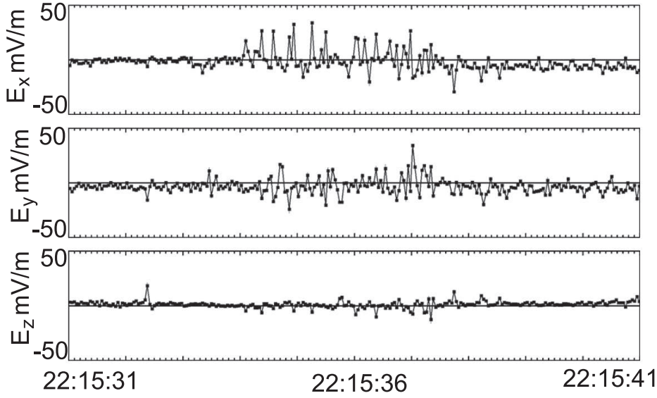
Fig. 23 Electric field measured onboard Cluster 2 satellite from 22:15:31 to 22:15:41. Electric field bursty spikes having amplitudes of 20\text{--}40\text{mVm}^{-1} having duration of the order of 0.1 sec are clearly seen during ramp crossing. Figure is provided by F. Mozer.
