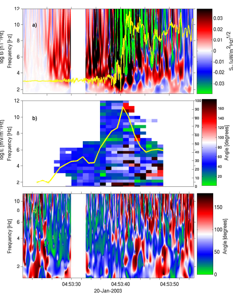
Fig. 16 Poynting flux in the Normal Incidence Frame (NIF) of the same shock as in Figure 15. a) Poynting flux S_{\parallel} projected on the local \mathbf{B}_0 in the NIF, where red corresponds to the upstream flux away from the shock. b) Angle \theta_{k,B} between \hat{\mathbf{k}} and magnetic field \mathbf{B}_0 . The yellow line represents the average over all frequencies (right scale). c) Angle between Poynting flux \mathbf{S} and \mathbf{B}_0 . (Adapted from Sundkvist et al. 2012)
