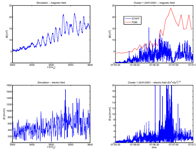
Fig. 34 Comparison of electric and magnetic fields observed on 24th of January 2001 by Cluster satellites and obtained in computer simulation by Comişel et al. (2011). Both panels show the fields in the vicinity of the foot/ramp regions. Top panels represent magnetic fields as measured by FGM instrument and STAFF search coil magnetometer (right), and obtained as a result of simulations(left). Bottom panels represent measured and simulated electric fields. One can see huge difference in amplitude of electric fields between measurements and simulations that results from artificial ratio of plasma to gyrofrequency and consequently unrealistic refractive index of waves. (Figure is provided by J. Soucek and H. Comişel)
