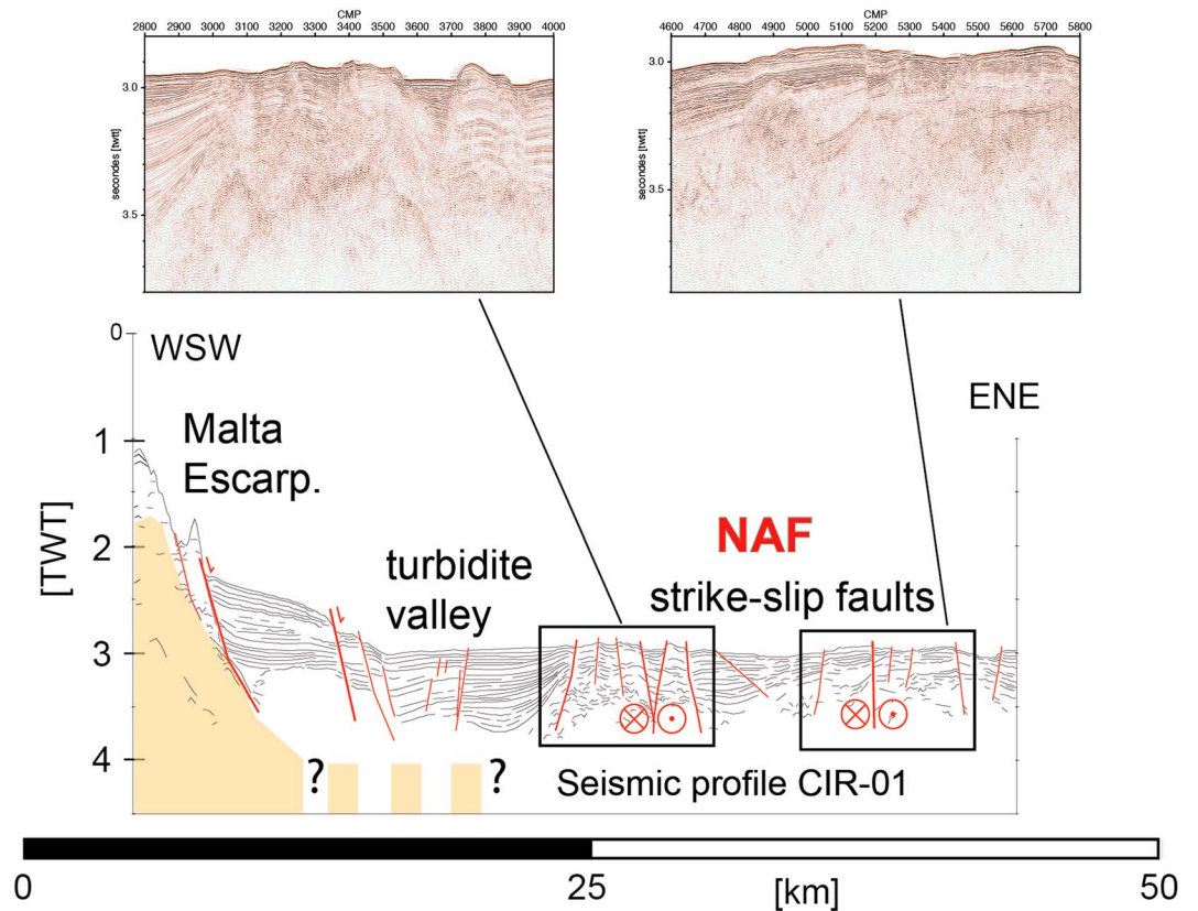
Figure 5. Seismic line CIR-01. Line drawing showing continental basement (orange shading, dashed when uncertain); and major interpreted faults (red lines with sense of motion). Boxes show zooms of the original 72 channel seismic data.
