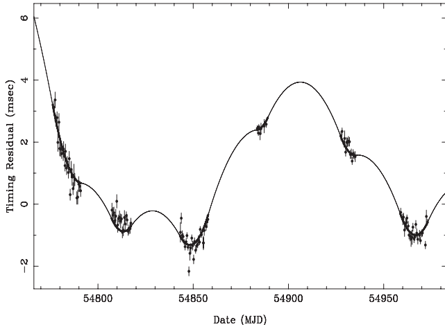
Figure 9. Least-squares weighted fit to timing residuals of PSR B1931+24 for observations in the range MJD \sim 54777 – 54973 . The timing residuals (filled circles) here are calculated with respect to a fixed \dot{\nu} ephemeris, while the fitted model (solid line) assumes two spin-down rates (see equation 2).
