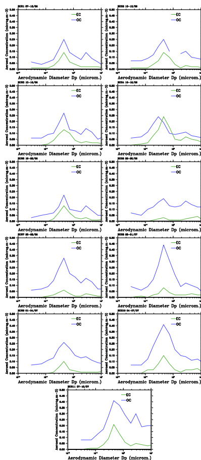
Figure 16. EC and OC (48 h-mean) aerosol mass size distributions obtained at Ersa from the impactor DEKATI instrument for all the SOP-1a period.
