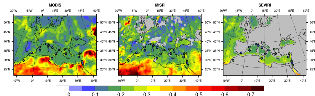
Figure 5. Total AOD (550 nm) obtained from the MODIS, MISR and SEVIRI (sea only) sensors for the June–July 2013 period. The AERONET/PHOTONS AOD is also indicated.
