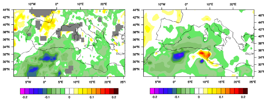
MISR observations
