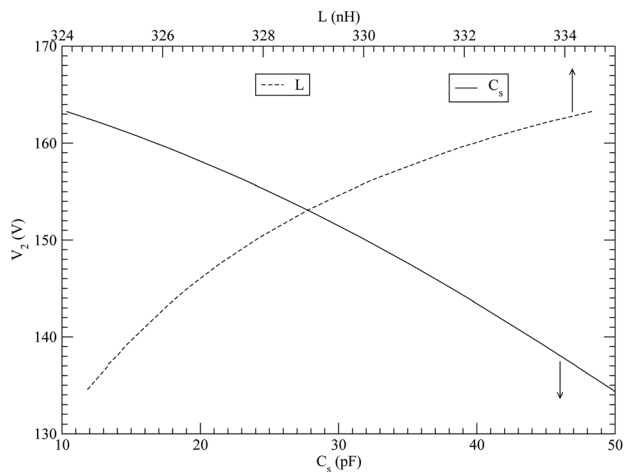
FIG. 8. Relationship between L , C_s , and \widehat{V}_2 for an optimized impedance matching.
