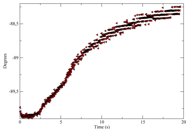
FIG. 12. (Color online) Current/voltage phase shift at the active electrode versus time.
