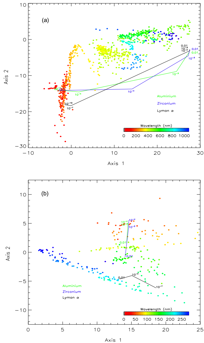
Fig. 2. 2-D representation of the variability of the solar irradiance (a) between 1 and 1000 nm, and (b) between 1 and 280 nm only. Various channels from the LYRA instrument are overlotted according to, the type of detector: silicon in (a) and diamond in (b). Each channel comes in several porosity levels, which are indicated next to the position of the channel.
