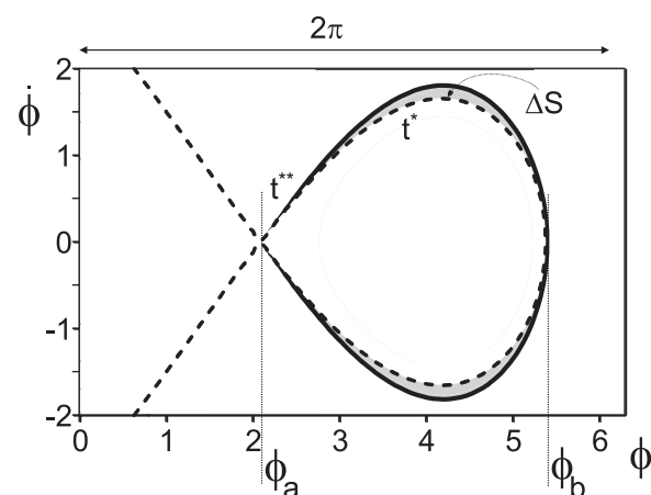
FIG. 11. Schematic view of the separatrix for two moments t^* , t^{**} . Grey color is used for the difference area surrounded by the separatrices.
