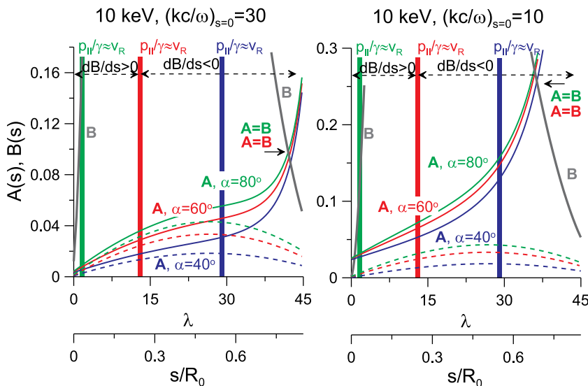
FIG. 15. The same as in Fig. 5, but for 10 keV.
