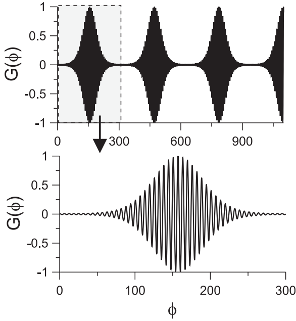
FIG. 3. Schematical view G(\phi) function.
