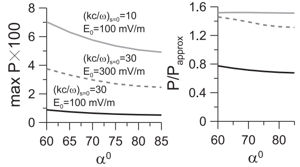
FIG. 13. Maximum value of probability as function of equatorial pitch-angle \alpha_0 for initial energy 100 keV. Right panel shows ratio of maxP and approximated value of probability P_{approx} .
