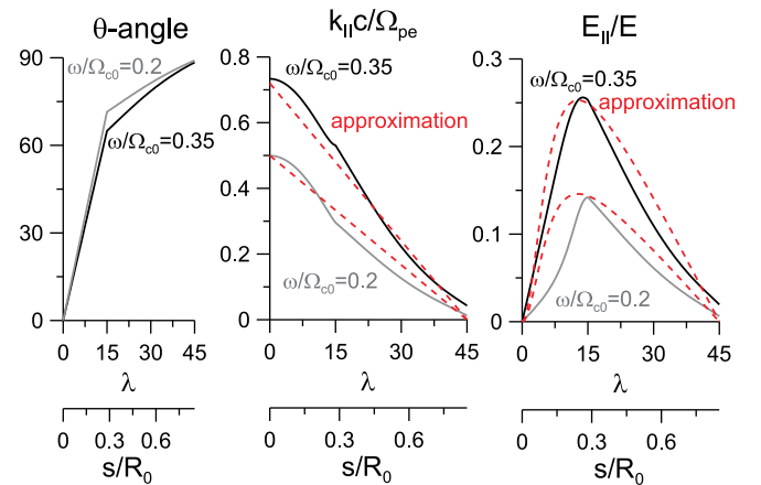
FIG. 2. Approximation of \theta as function of magnetic latitude is shown in left panel. Central panel shows the parallel component of wavevector k_{||} and the corresponding approximation (red color). Right panel shows the normalized parallel component of electric field E_{||}/E and the corresponding approximation (red color).
