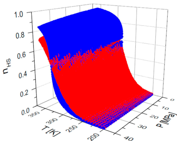
Figure 4. Simulated HS fractions as a function of temperature and pressure variations for two values of the interaction parameter (red— \Gamma/k_B = 160 K and blue— \Gamma/k_B = 300 K). The calculation parameters are: \Delta'/k_B = 1978.6 K, \ln(g) = 6.906 , \delta V = 100 \text{ \AA}^3 .
