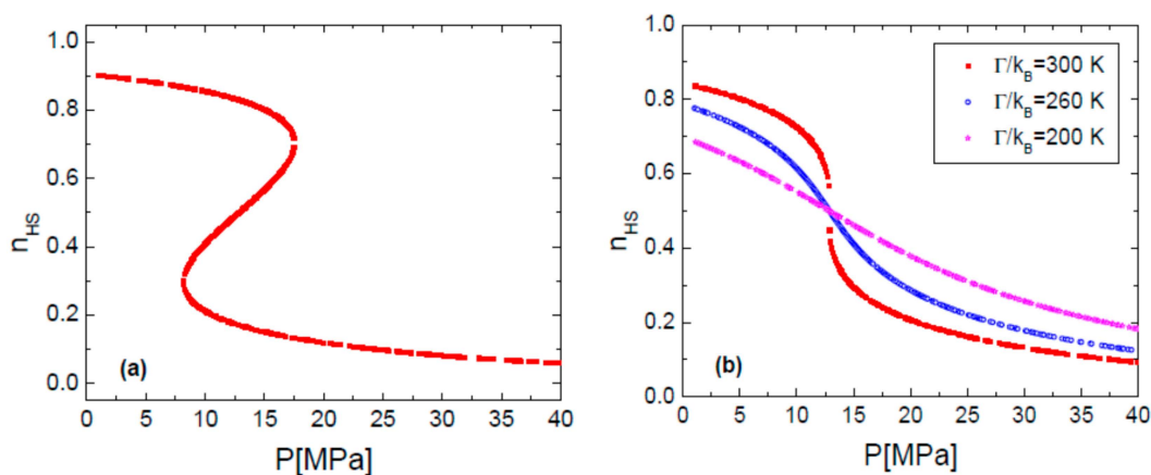
Figure 3. Simulated HS fraction n_{\text{HS}} vs. pressure for (a) \Gamma/k_{\text{B}} = 360 K and (b) for different values of \Gamma ; The calculation parameters are: \Delta'/k_{\text{B}} = 1978.6 K, \ln(g) = 6.906 , \delta V = 100 \text{ \AA}^3 , T = 300 K.
