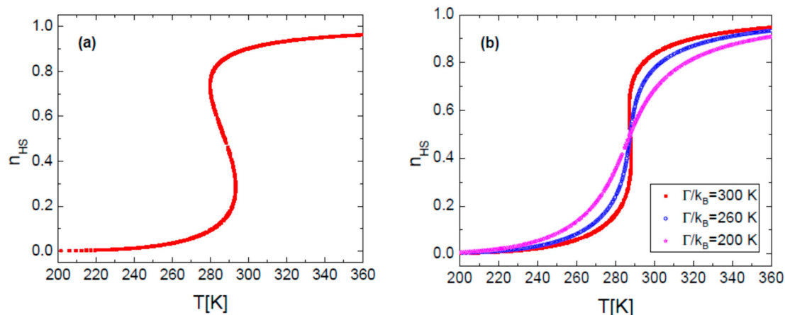
Figure 2. (a) Simulated HS fraction n_{\text{HS}} vs. temperature for \Gamma/k_{\text{B}} = 360 K; (b) Simulated HS fraction n_{\text{HS}} vs. temperature for different values of interaction parameter. The calculation parameters are: \Delta'/k_{\text{B}} = 1978.6 K, \ln(g) = 6.906 , \delta V = 100 \text{ \AA}^3 , p = 0.1 MPa.
