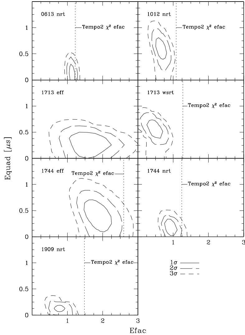
Figure A1. The marginalized posteriors of all data sets, as a function of the EFAC and EQUAD parameters. The contours are at the 1 \sigma , 2 \sigma and 3 \sigma level, indicating a respective volume inside that region of 68, 95 and 99.7 per cent. For the J1713-0747 posterior, the TEMPO2 \chi^2 estimate is not shown because it has the off-scale value of 4.4.
