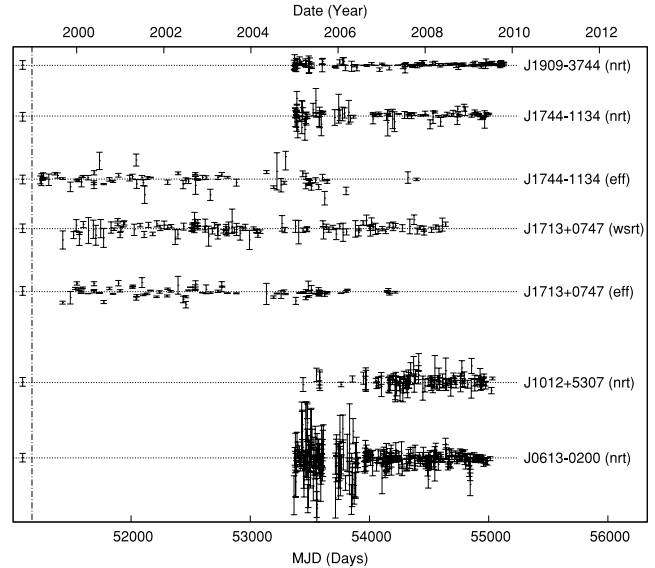
Figure 2. The timing residuals of all the pulsars used in the GWB limit calculation. The time in MJD is shown on the x -axis. On the left of the dot-dashed line we have placed a sample residual with an uncertainty of 1 \mu\text{s} .
