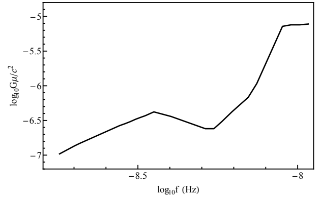
Figure 17. The cosmic string tension upper limits in the case of p = 1 , obtained from the sensitivity curve presented in Fig. 13 for a range of the probed frequencies. For these limits, only the information about the amplitude of the GWB has been used. The most stringent constraint is given by the lowest frequency probed, whereas results for frequencies higher than \sim 10^{-8} \text{ Hz} have been omitted, since already for frequencies \gtrsim 7 \times 10^{-9} \text{ Hz} the tension upper limits are unphysically high.
