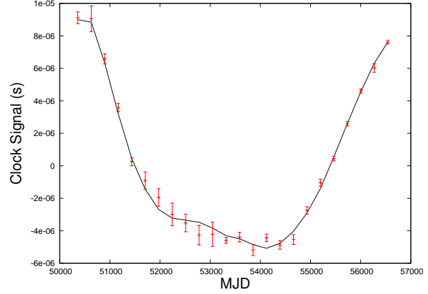
Figure 2. Simulated clock error used in our analysis (black line) after subtracting the maximum likelihood timing models from the joint analysis, and the time averaged maximum likelihood recovered clock signal with 1\sigma uncertainties (red points with error bars). We find the recovered signal is consistent with the injected signal across the whole dataspan.
